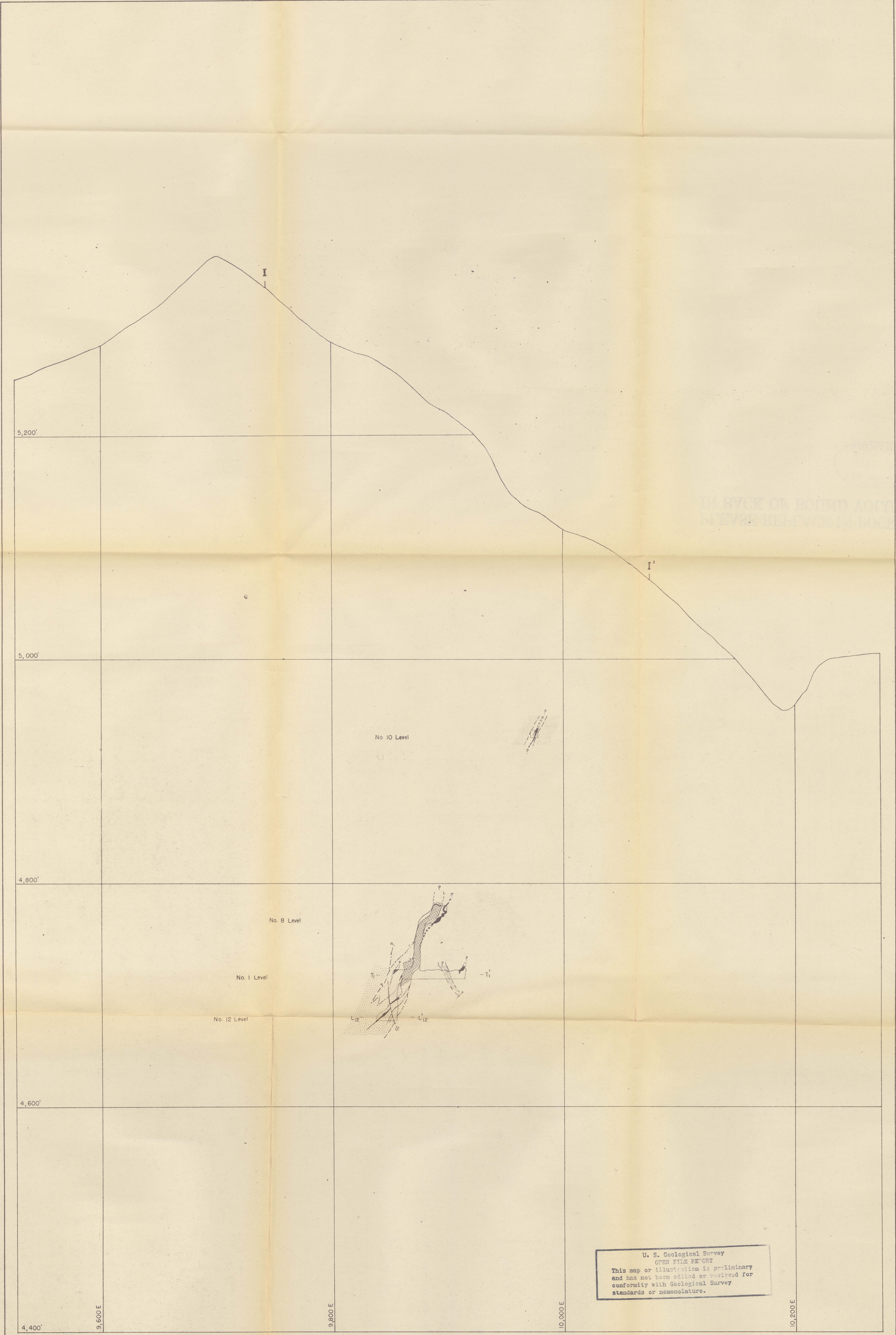
GEOLOGIC SECTION I-I', BLUE LEDGE MINE, SISKIYOU COUNTY, CALIFORNIA
