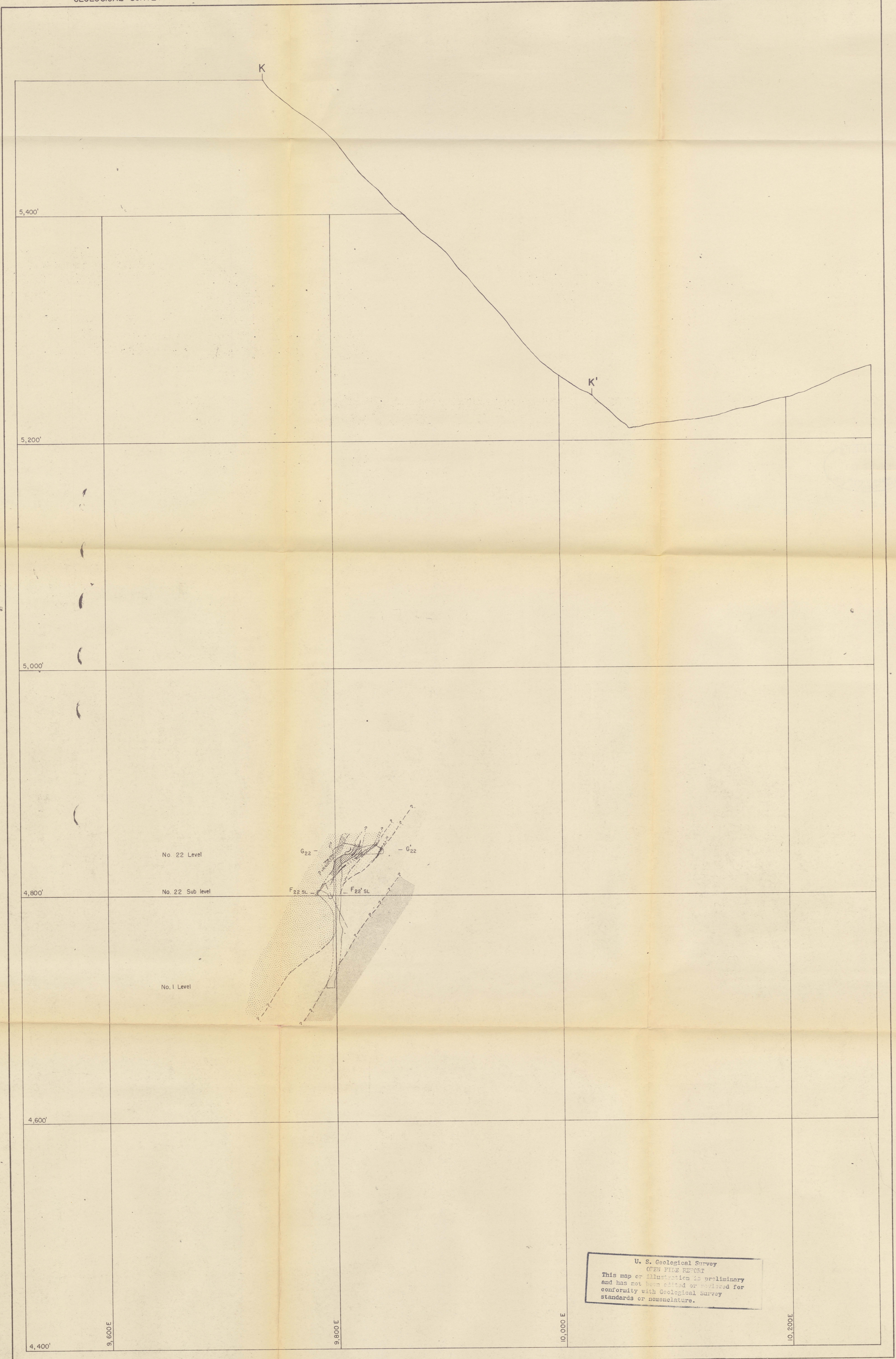
GEOLOGIC SECTION K-K', BLUE LEDGE MINE, SISKIYOU COUNTY, CALIFORNIA
