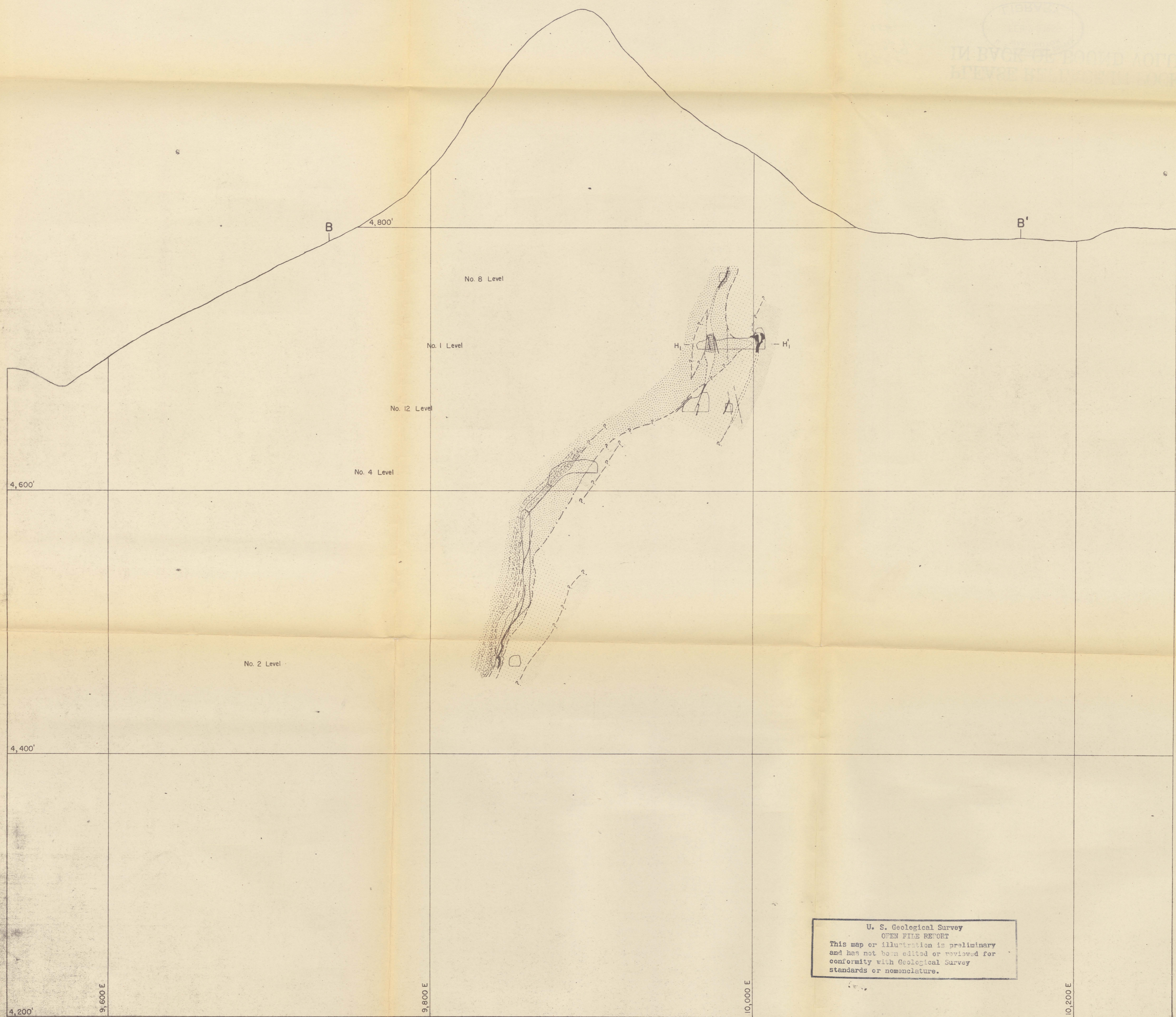
GEOLOGIC SECTION B-B', BLUE LEDGE MINE, SISKIYOU COUNTY, CALIFORNIA
