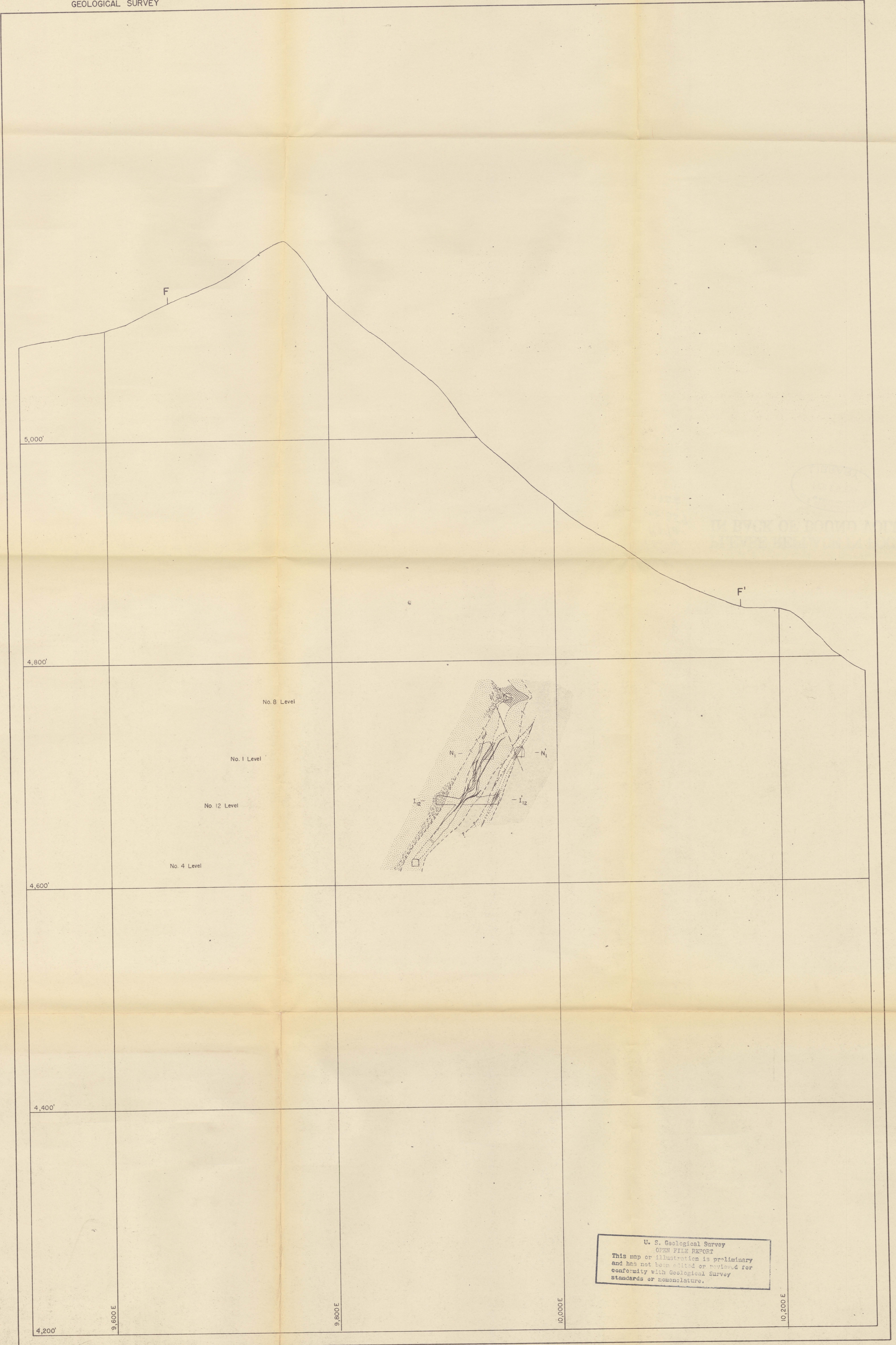
GEOLOGIC SECTION F-F', BLUE LEDGE MINE, SISKIYOU COUNTY, CALIFORNIA
