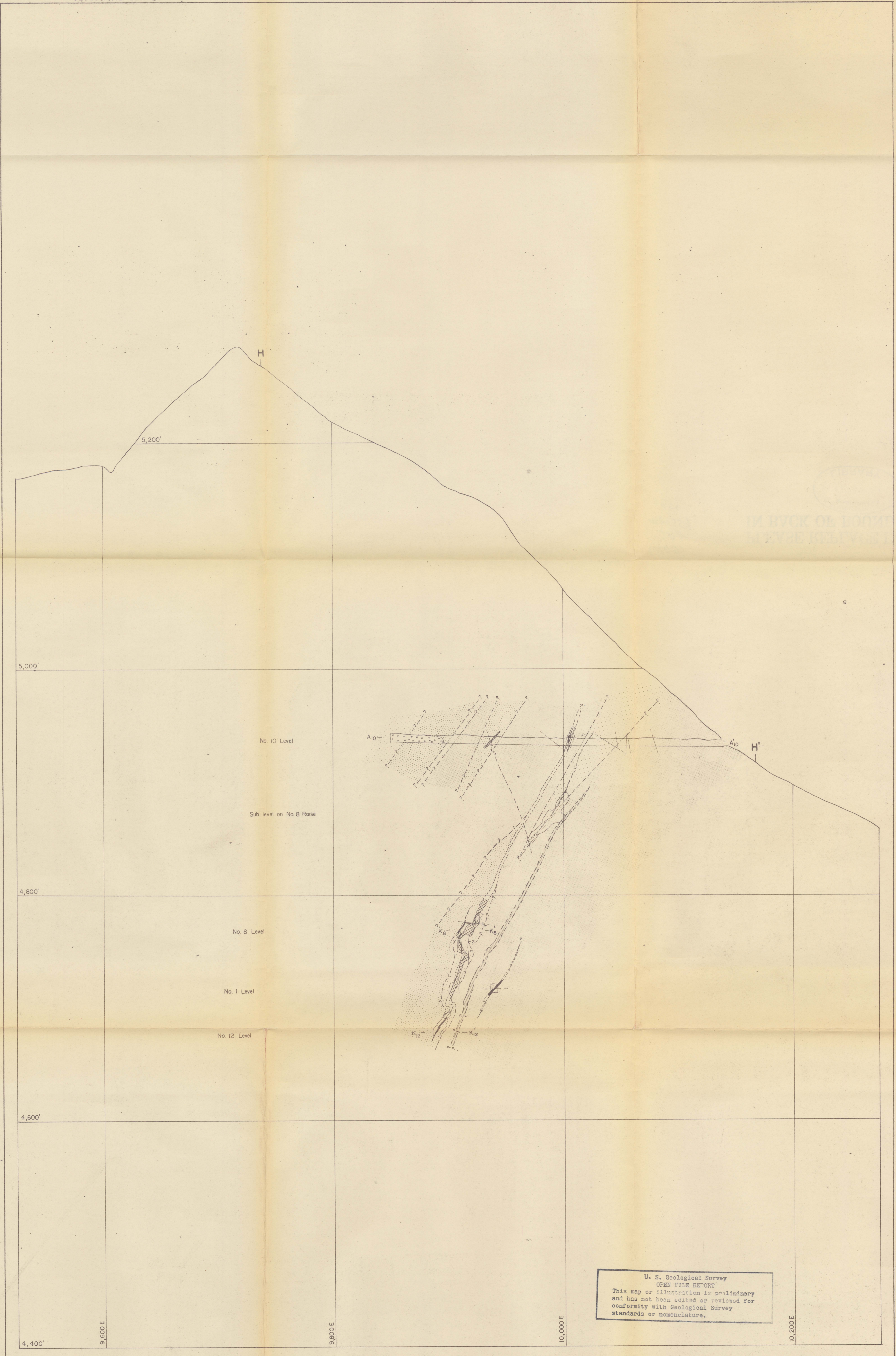
GEOLOGIC SECTION H-H', BLUE LEDGE MINE, SISKIYOU COUNTY, CALIFORNIA
