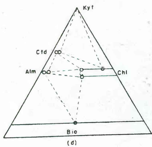
Phase Diagrams, showing mineral assemblages of quartz and muscovite schist stable at successively higher metamorphic grades in Hyde Park quadrangle. Construction of the diagrams is explained in the text and on Figure 5.
