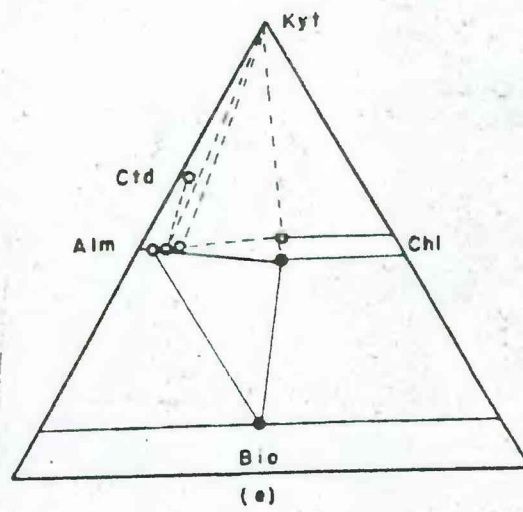
Phase Diagrams, showing mineral assemblages of quartz and muscovite schist stable at successively higher metamorphic grades in Hyde Park quadrangle. Construction of the diagrams is explained in the text and on Figure 5.
