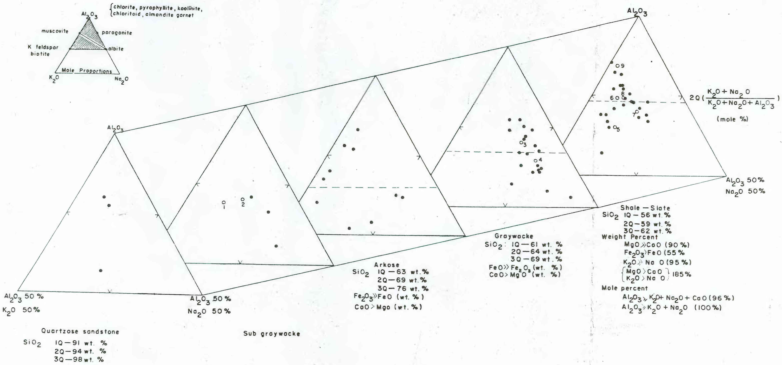
Chemical characteristics of argillaceous-arenaceous sedimentary rocks
