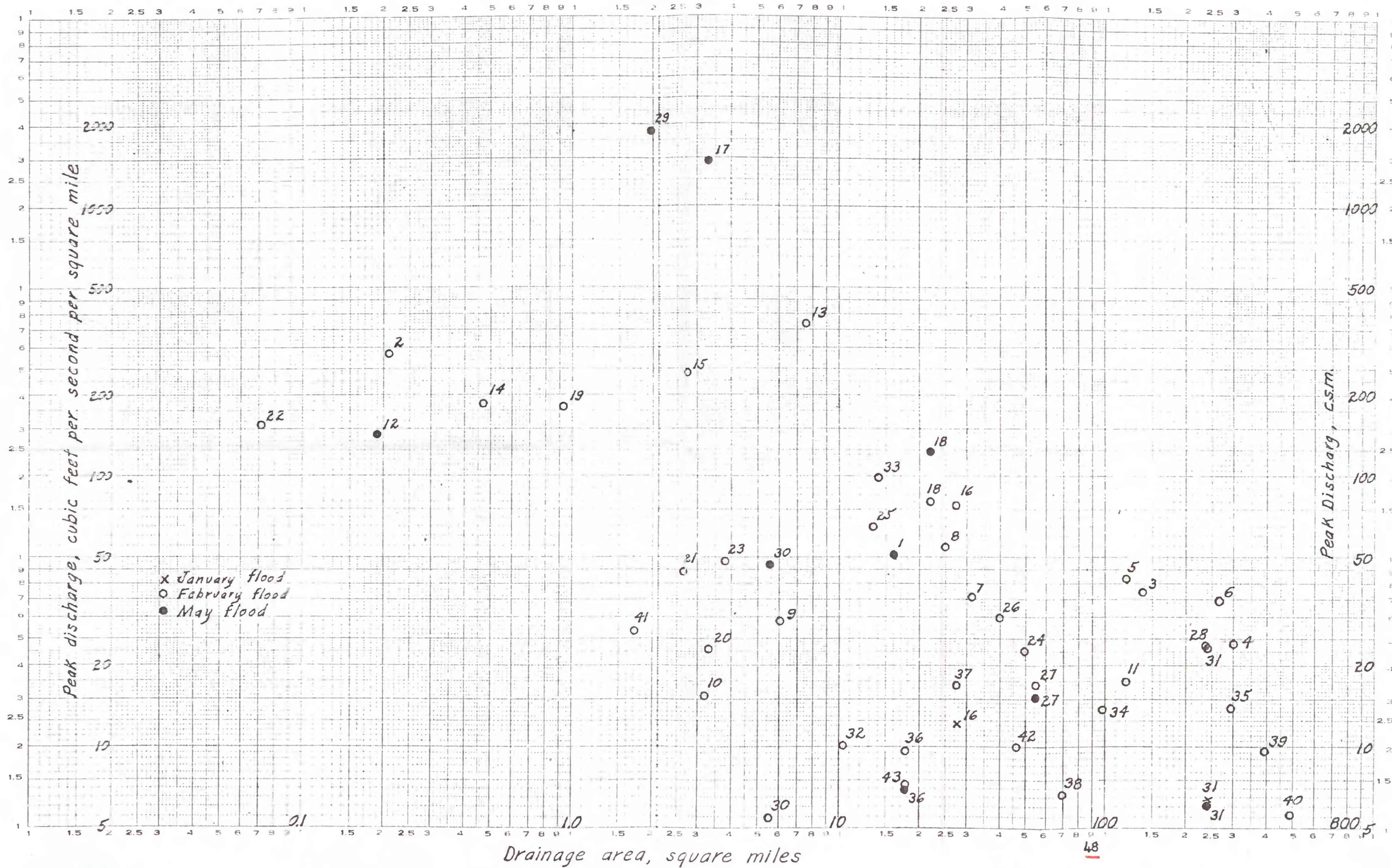
Figure 14.-- Relation of unit discharge to size of drainage area
