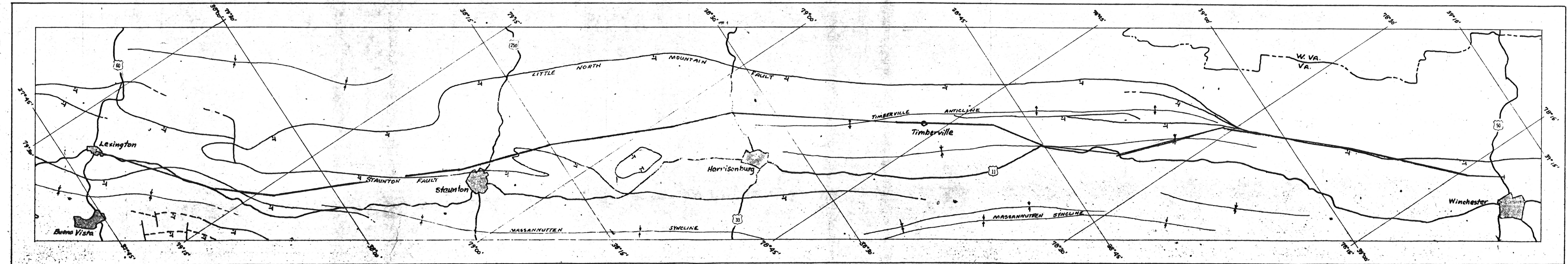
Fig. 2 REGIONAL AEROMAGNETIC PROFILE, WINCHESTER TO LEXINGTON, VIRGINIA
