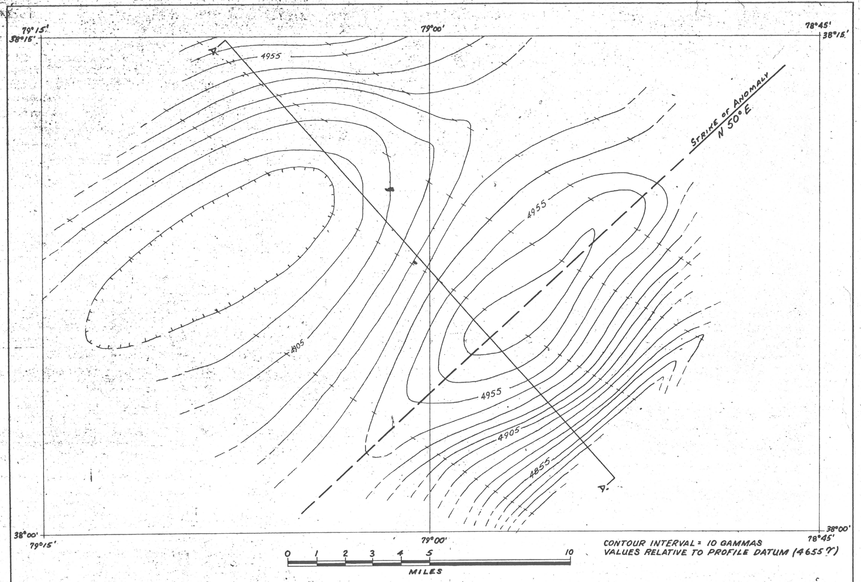
A. Regional Total Intensity Aeromagnetic Configuration of the Staunton and Waynesboro Quadrangles, Va. showing the Fishersville Anomaly and location of the profile used for depth calculation.
