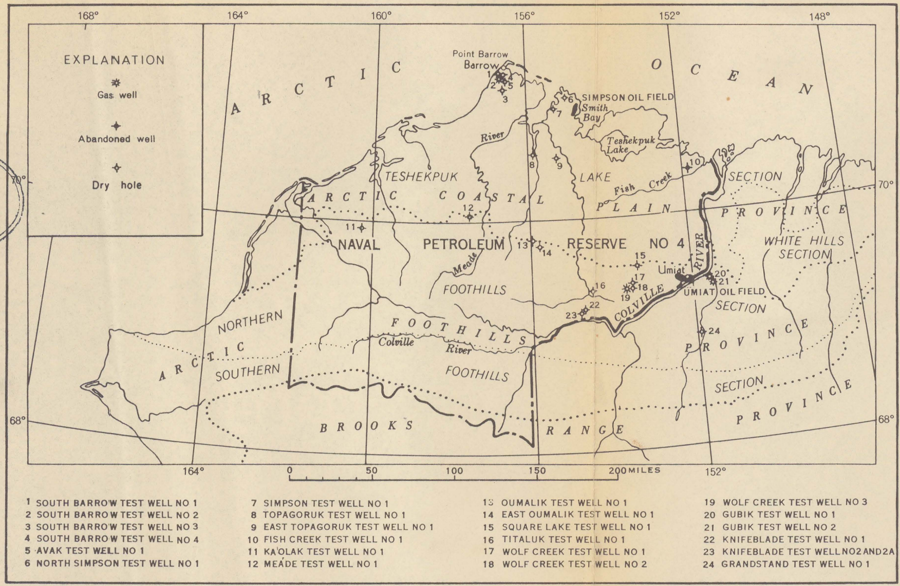
Figure 3. - Index map of northern Alaska showing location of test wells and oil fields
