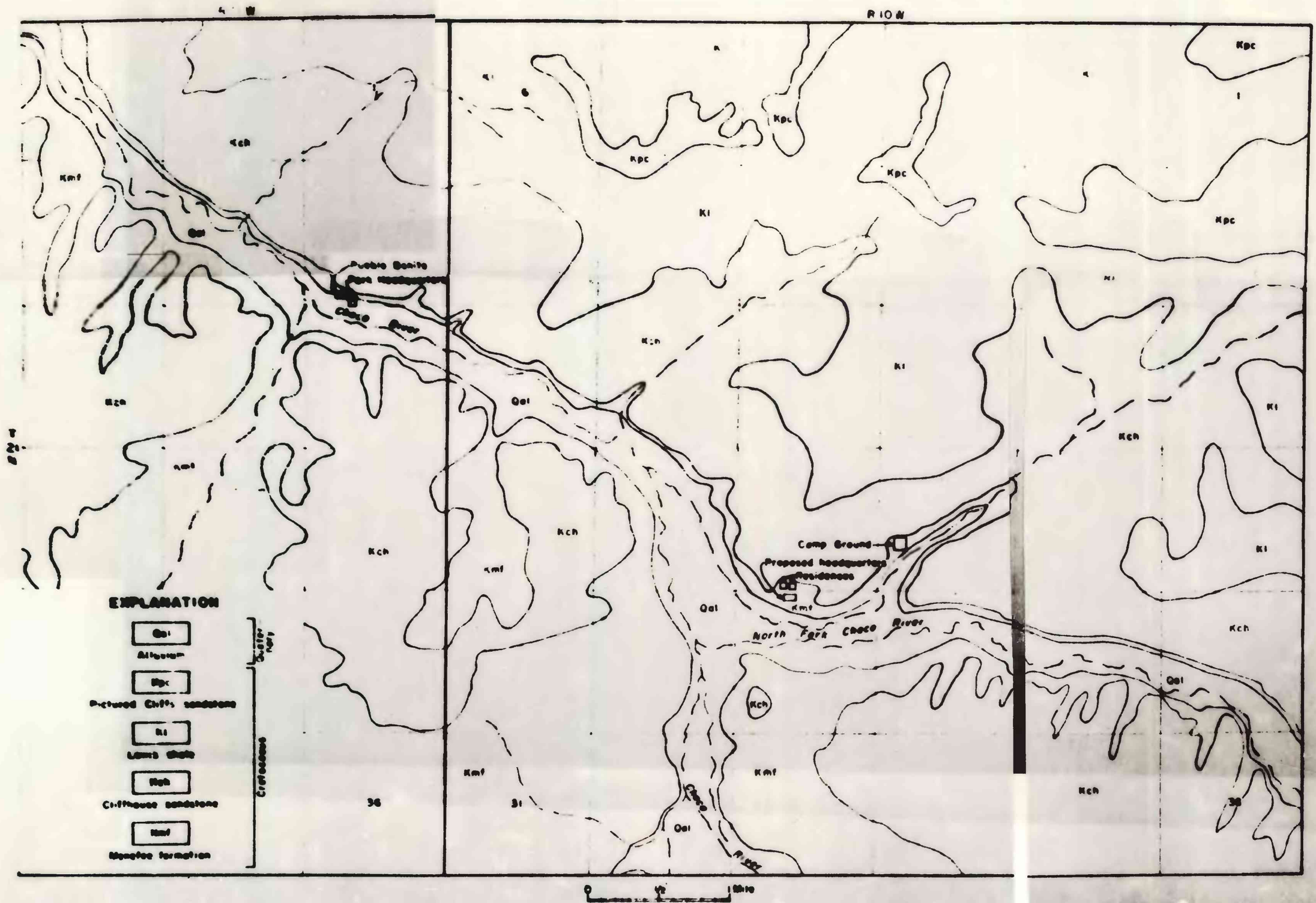
Plate I.—Geologic map of the Chaco Canyon National Monument headquarters area, New Mexico
