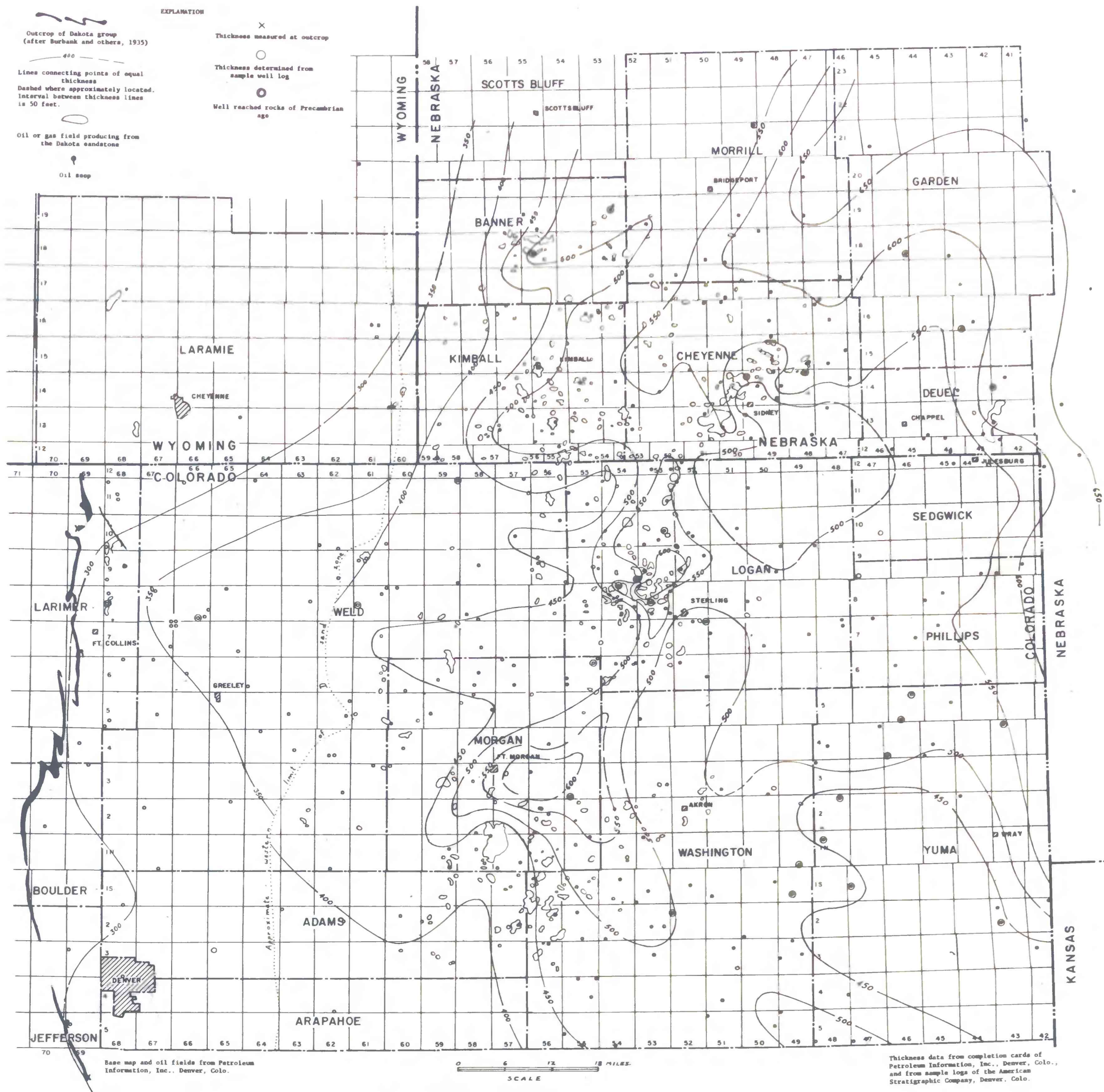
FIGURE 3. Thickness map of the Dakota sandstone in part of the Denver basin.
