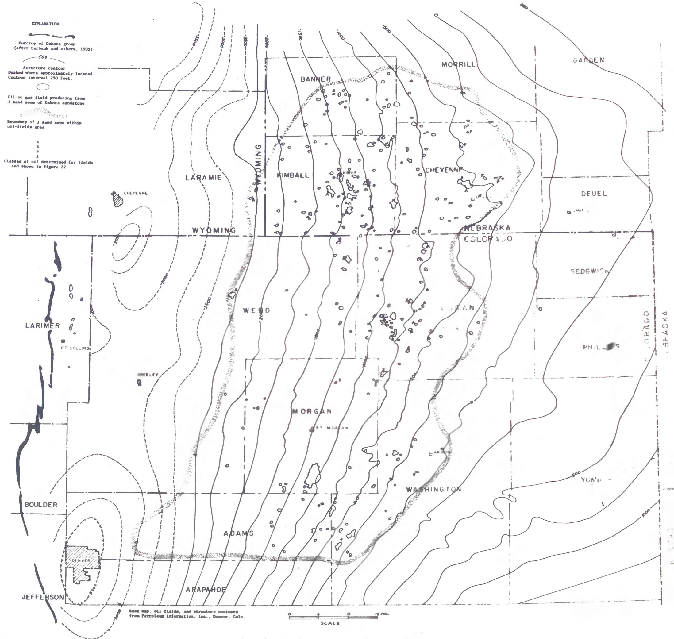
FIGURE 6. Map of oil and gas fields in the J sand zone of the Dakota sandstone in part of the Denver basin showing generalized structure contours drawn on the top of the J sand zone.
