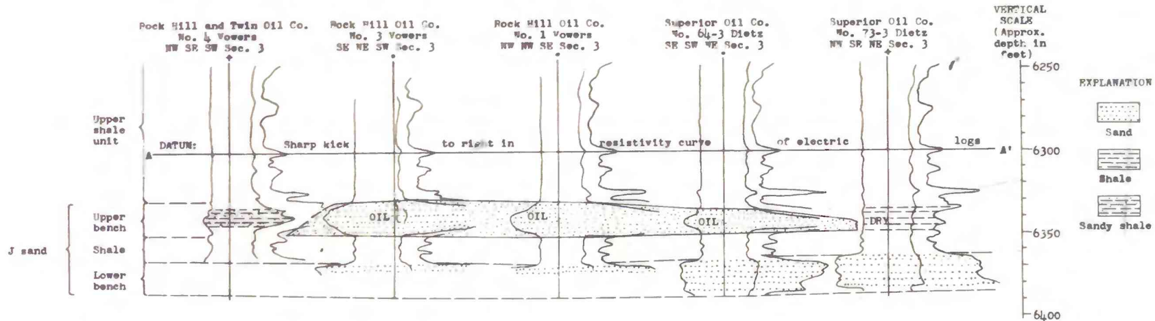
FIGURE 12. Cross section of the J sand zone of the Dakots sandstone in the Dietz oil field. T. 13 N., R. 55 W., Kimball County, Nebraska. See figure 13 for line of cross section.
