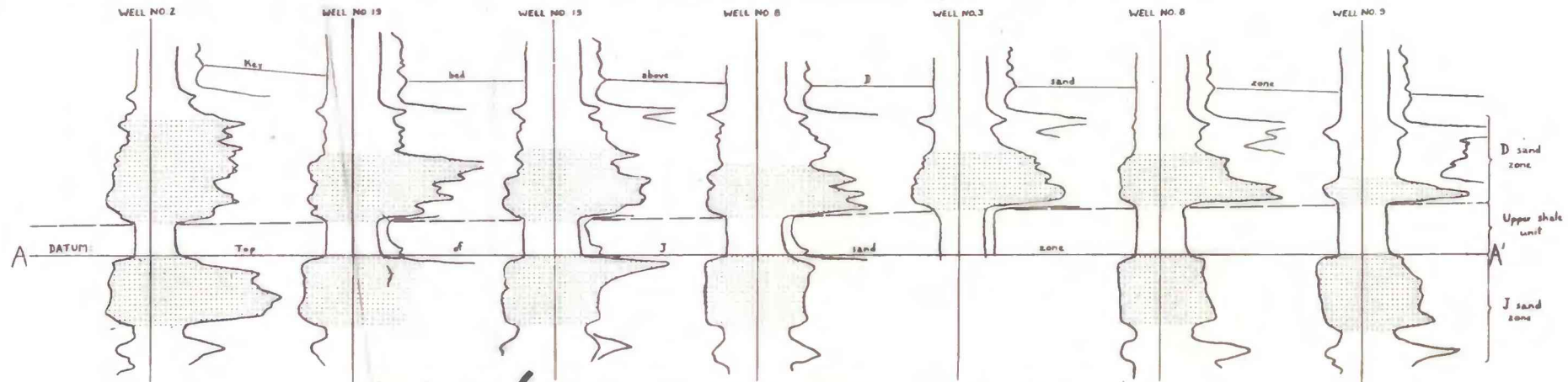
Cross section of sand zones of the Dakota sandstone in the Badger Creek field, T. 2 S., R. 57 W., Adams County, Colorado. Logs aligned on top of J sand zone.
