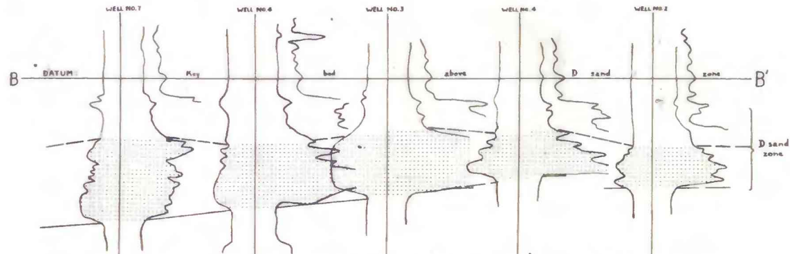
Cross section of sand zone of the Dakota sandstone in the Bobcat field, T. 15 N., R. 56 W., Washington County, Colorado. Logs aligned on key bed above D sand zone.
