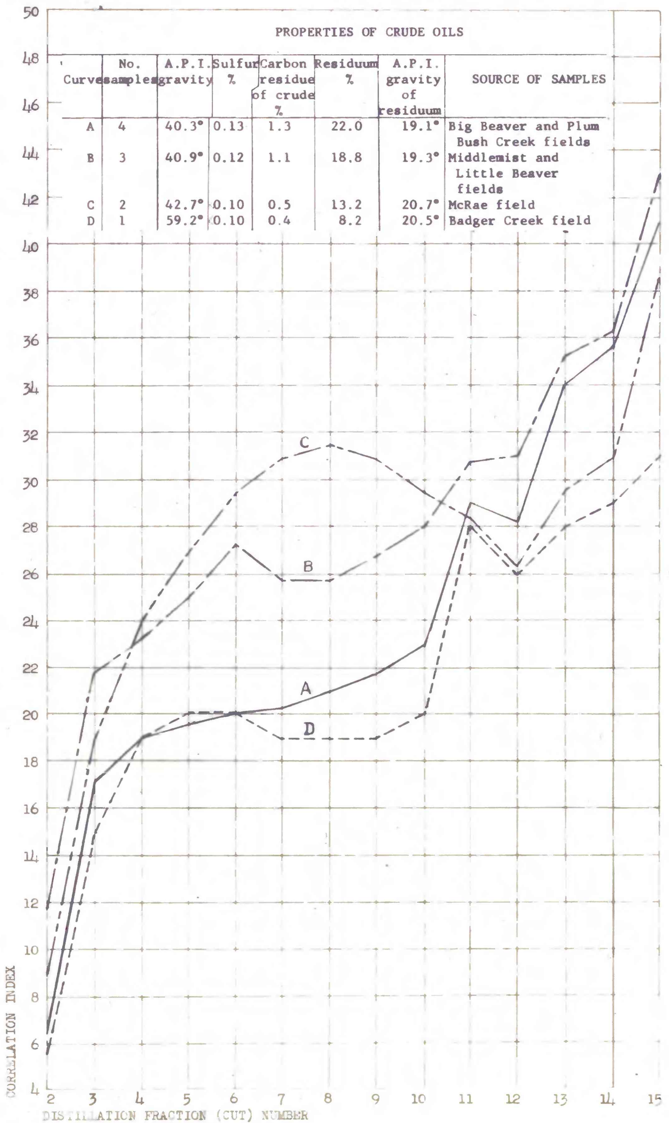
FIGURE 21. Curves showing correlation indexes of crude oils in the J sand in selected oil fields in the southern part of the oil-fields area of the Denver basin. See figure 10 for location of fields.
