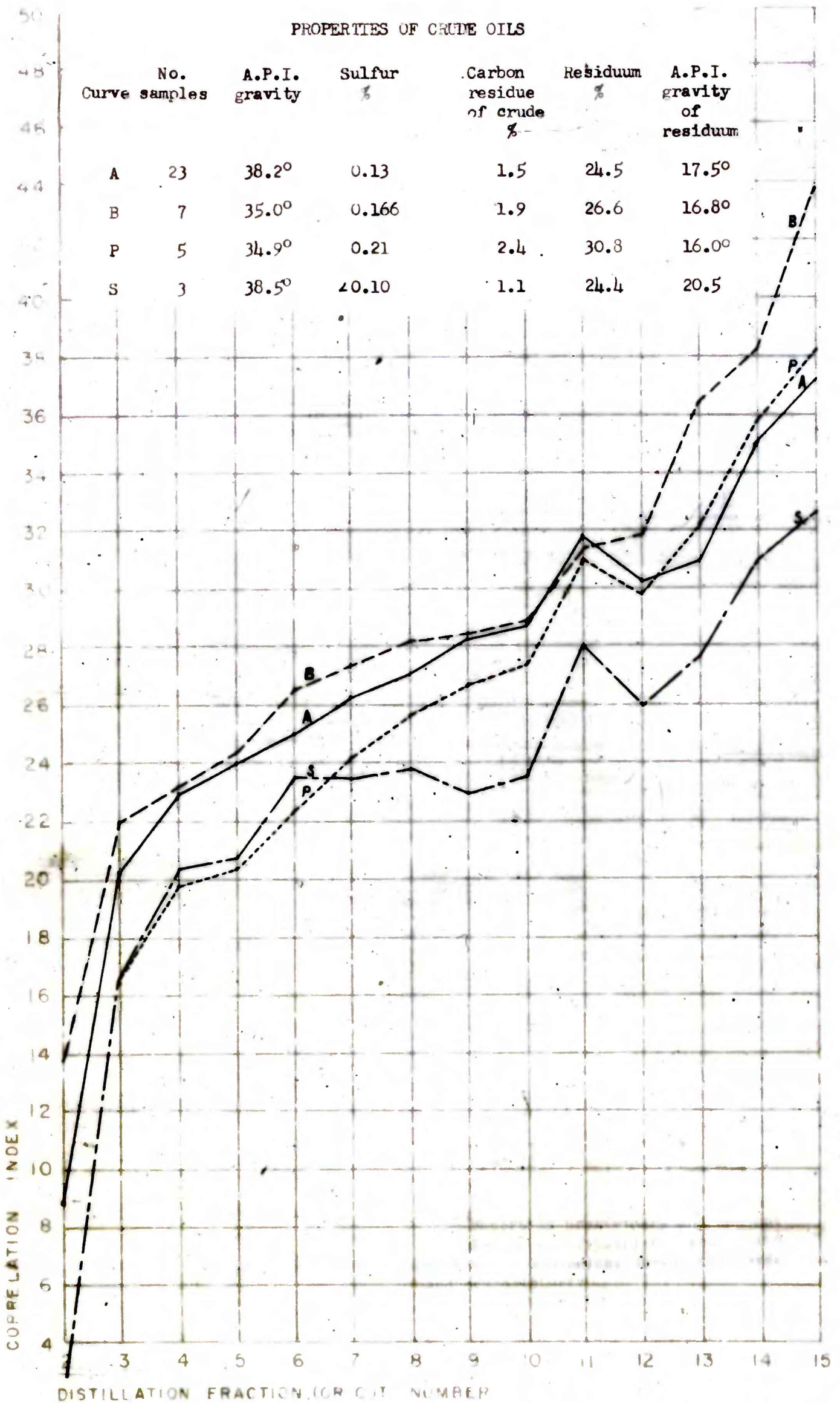
FIGURE 22. Curves showing correlation indexes of crude oils in the J sand in selected oil fields in the oil-fields area of the Denver basin. See figure 6 for locations of fields.
