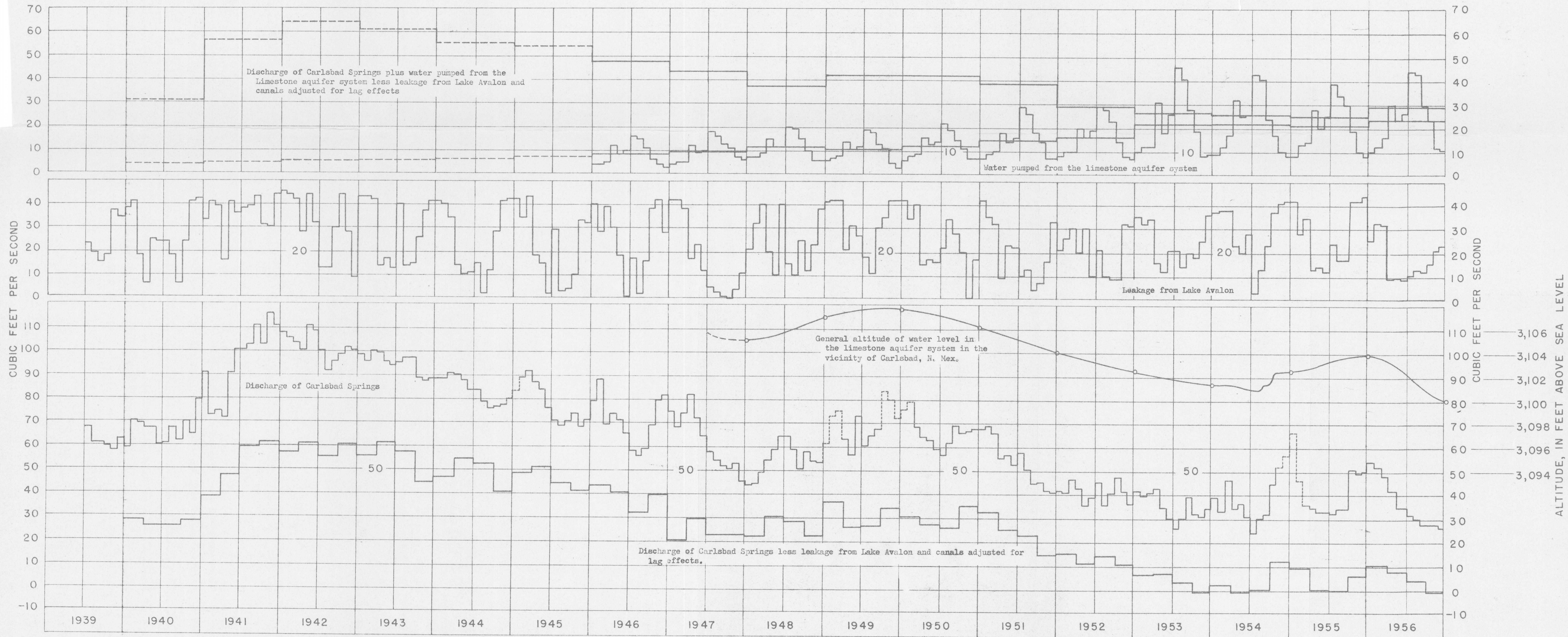
Figure 4.--Discharge of Carlsbad Springs, leakage from Lake Avalon, water pumped from the limestone aquifer system, contribution to flow from Carlsbad Springs from sources other than leakage from Lake Avalon and canals, and annual discharge from the limestone aquifer system less leakage from Lake Avalon and canals in the vicinity of Carlsbad, New Mexico
