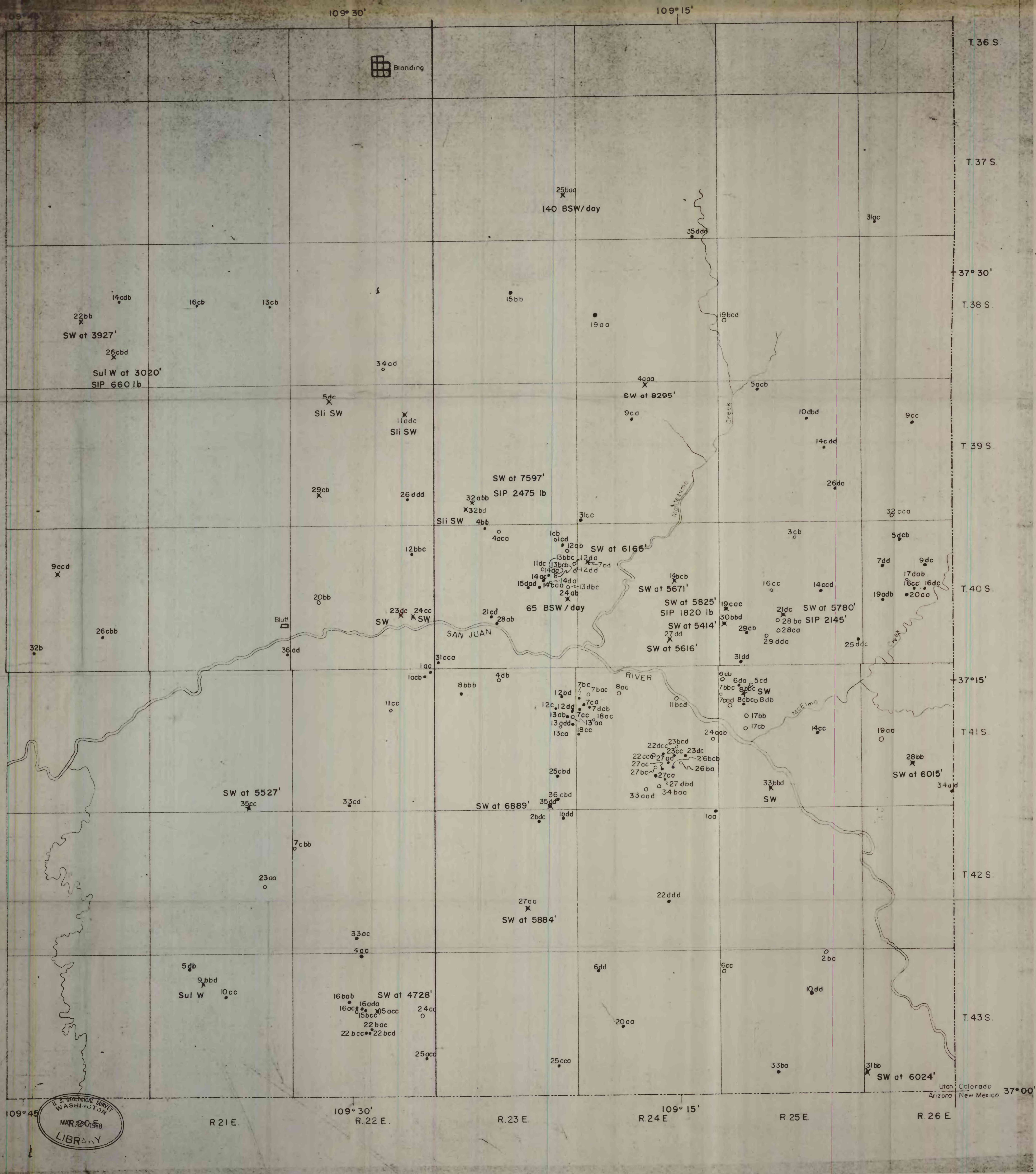
FIGURE 2. MAP SHOWING LOCATION OF OIL WELLS IN SOUTHEASTERN UTAH, AS OF JULY 1957 (IN CENTER OF ANETH FIELD-T.40S., R.24E.-ONLY SELECTED WELLS ARE SHOWN)
