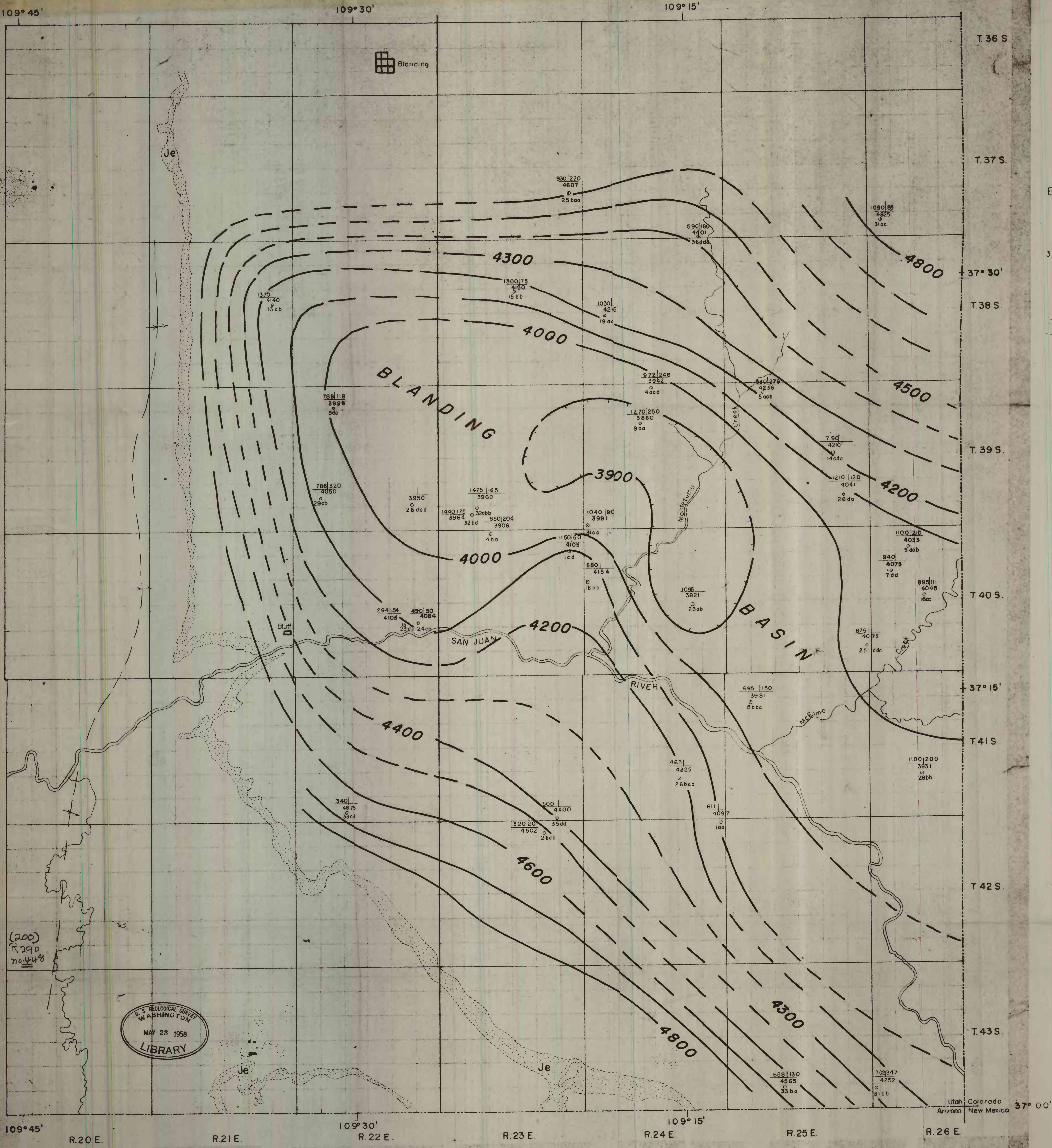
FIGURE 9. MAP SHOWING STRUCTURE AT THE BASE OF THE ENTRADA SANDSTONE IN SOUTHEASTERN UTAH
