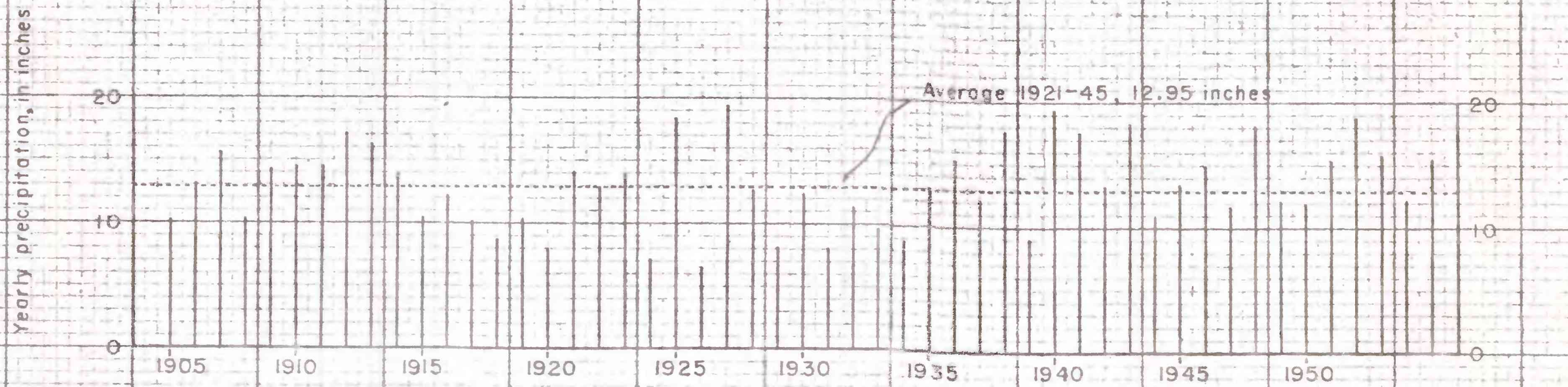
PRECIPITATION AT KLAMATH FALLS DURING CLIMATIC YEARS ENDING SEPTEMBER 30 OF EACH YEAR, 1905-55
