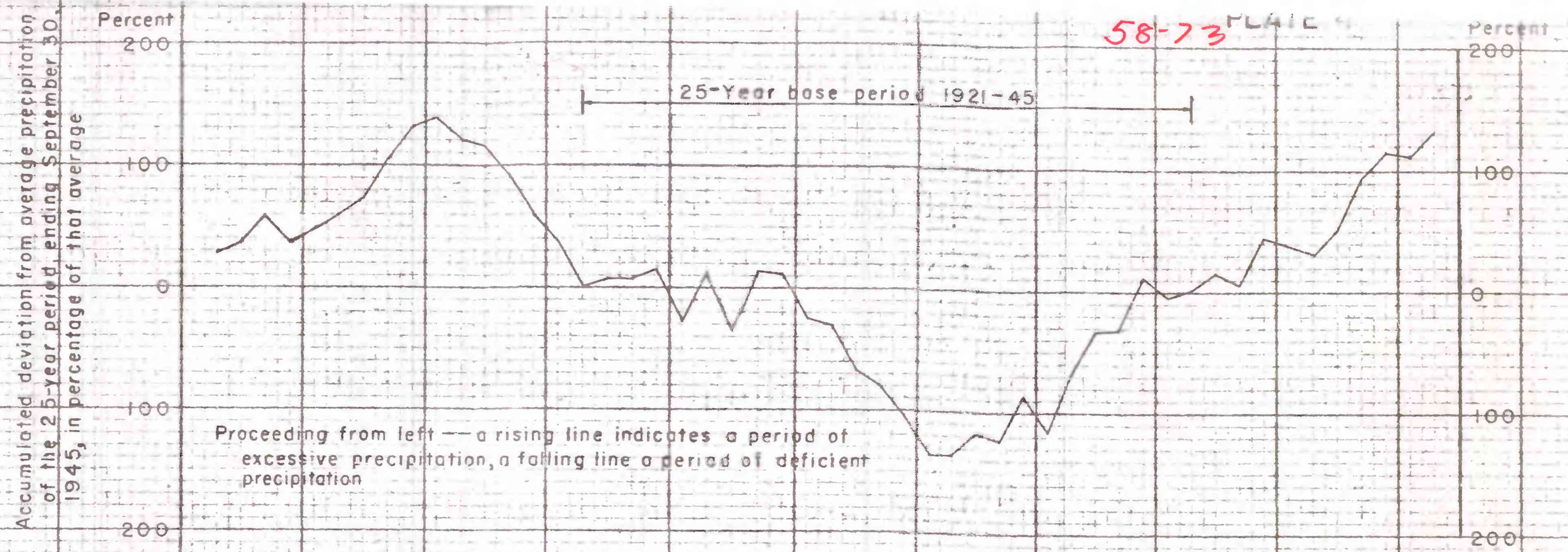
ACCUMULATED DEVIATION IN PERCENTAGE OF THE YEARLY AVERAGE PRECIPITATION FOR THE 25-YEAR PERIOD OCTOBER 1, 1920 - SEPTEMBER 30, 1945, AT KLAMATH FALLS
