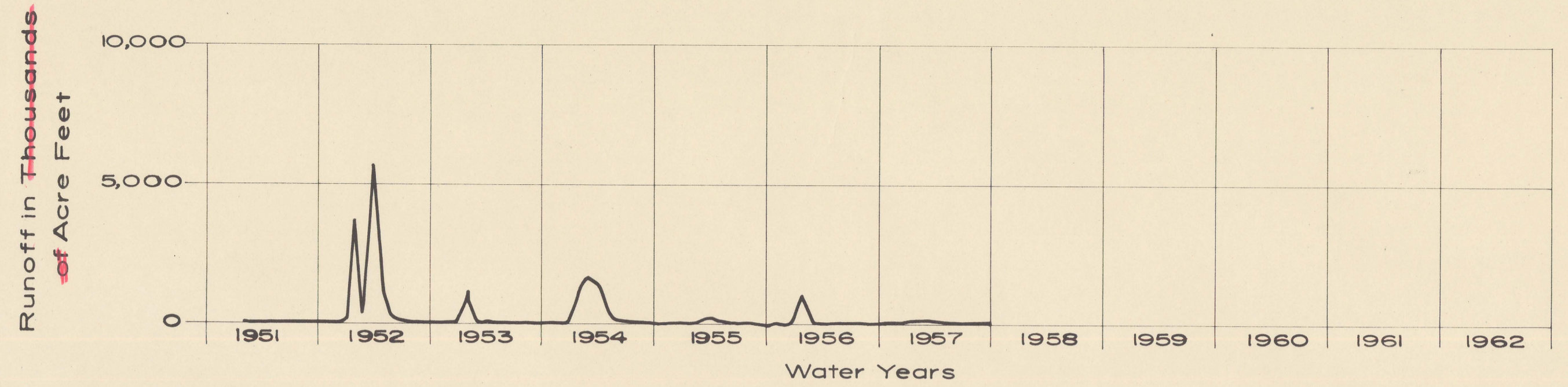
HYDROGRAPH OF MONTHLY RUNOFF OF DE LUZ CREEK
