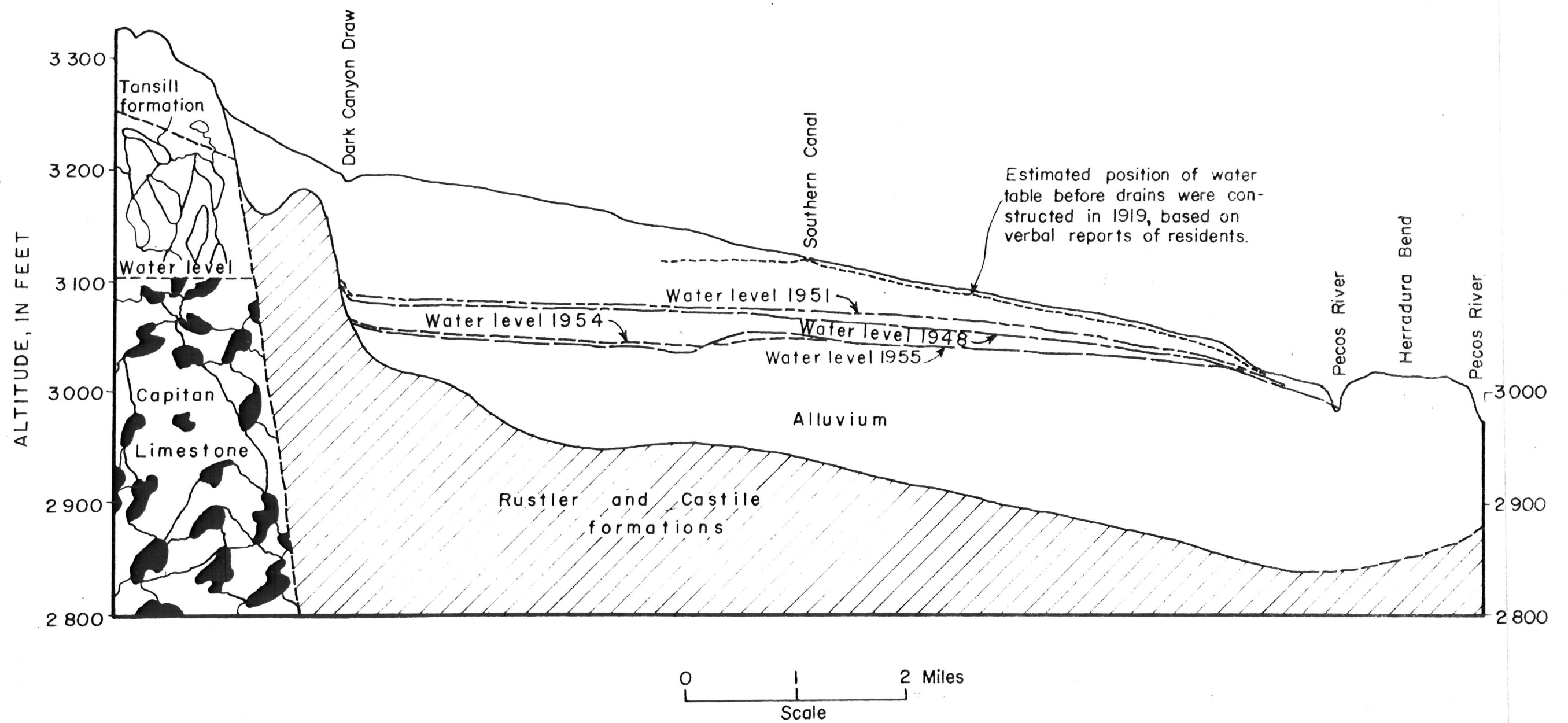
Figure 36.--Map and cross section of part of the Pecos River valley south of Carlsbad, Eddy County, N. Mex., showing geology and changes in water level.
