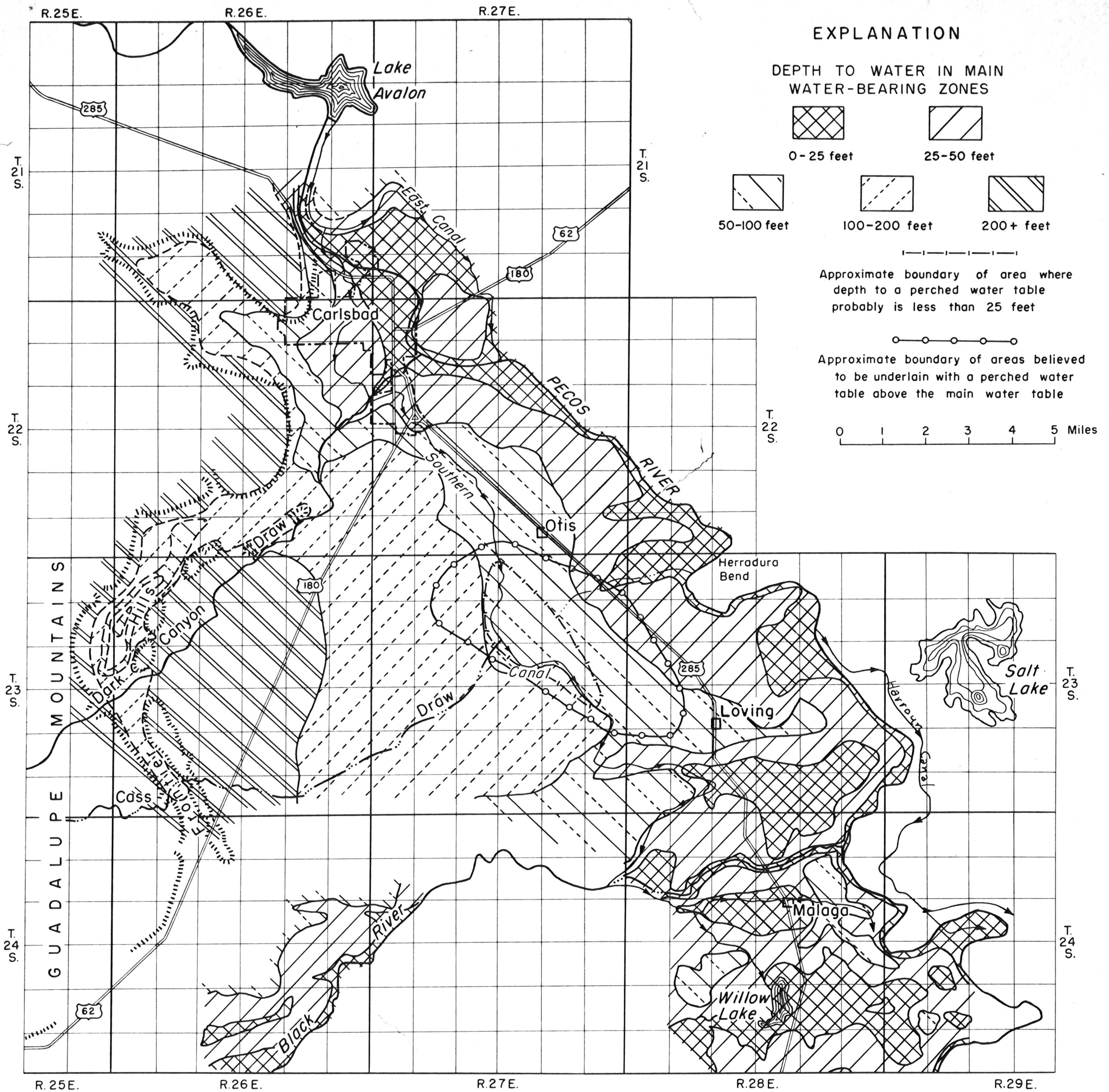
Figure 31.--Map of part of Eddy County, N. Mex., showing depths to the water table or piezometric surface, January 1955.
