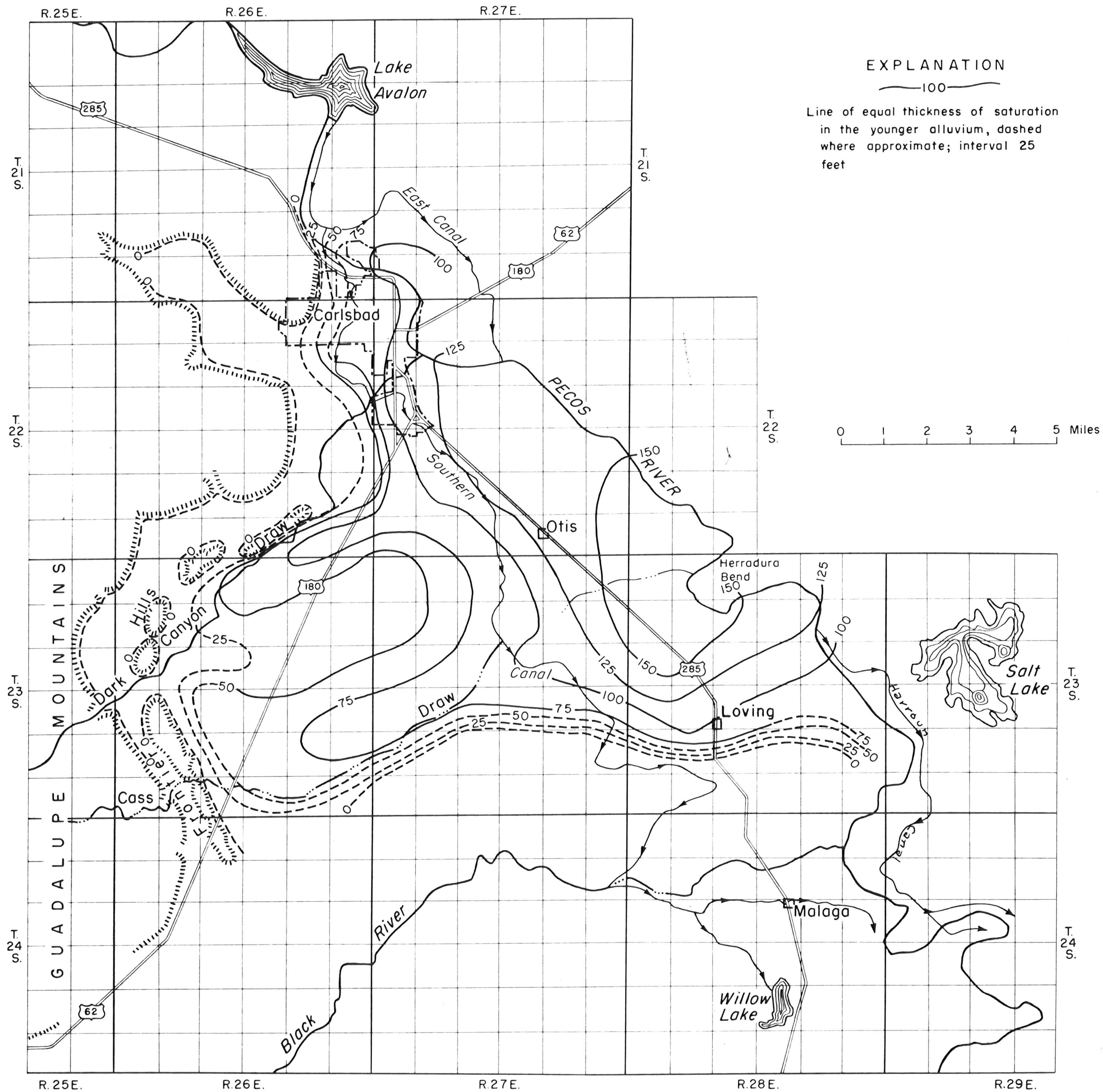
Figure 30.--Map showing saturated thickness of the alluvium south of Carlsbad, Eddy County, N. Mex., during January 1955; prepared by superimposing water-table contours (fig. 35) upon the base-of-alluvium contours (fig. 16).
