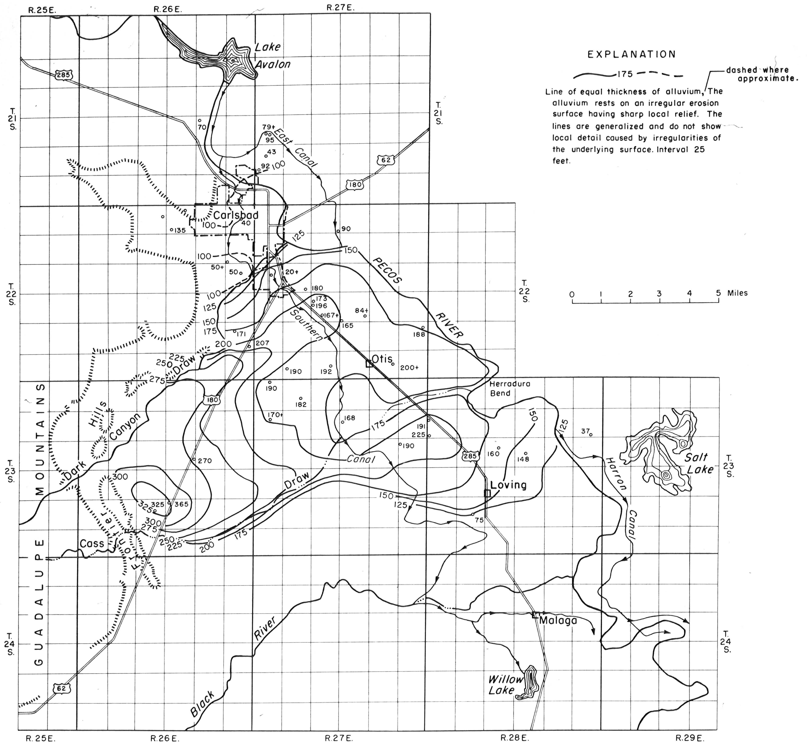
Figure 15.--Map showing approximate thickness of alluvium south of Carlsbad, Eddy County, N. Mex.; prepared by superimposing land-surface contour lines as shown on U.S.G.S. topographic maps upon the base-of-alluvium contour lines (fig. 16).
