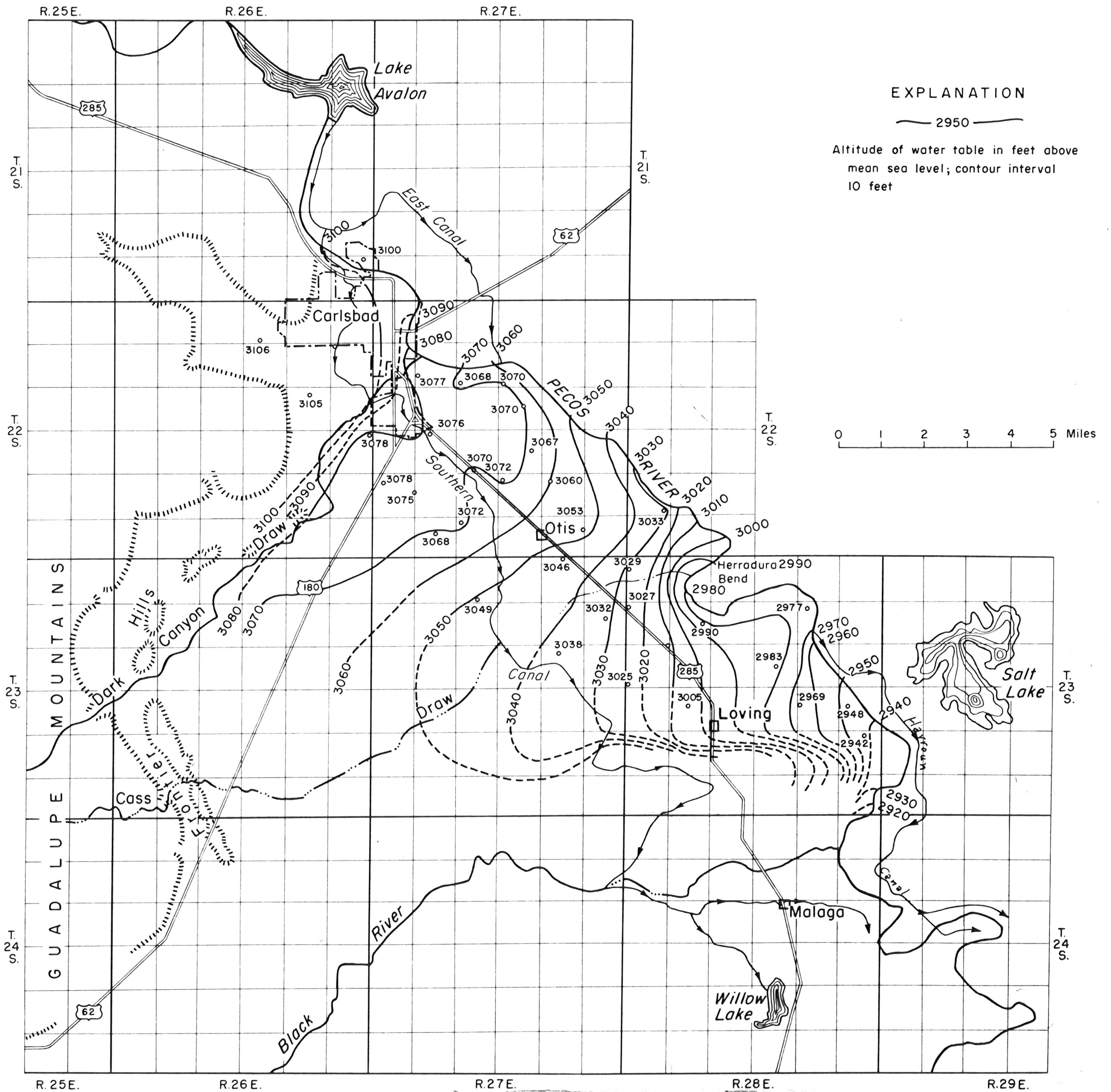
Figure 32.—Map showing configuration of the main water table in the alluvium of the Pecos River valley south of Carlsbad, Eddy County, N. Mex., during January 1948.
