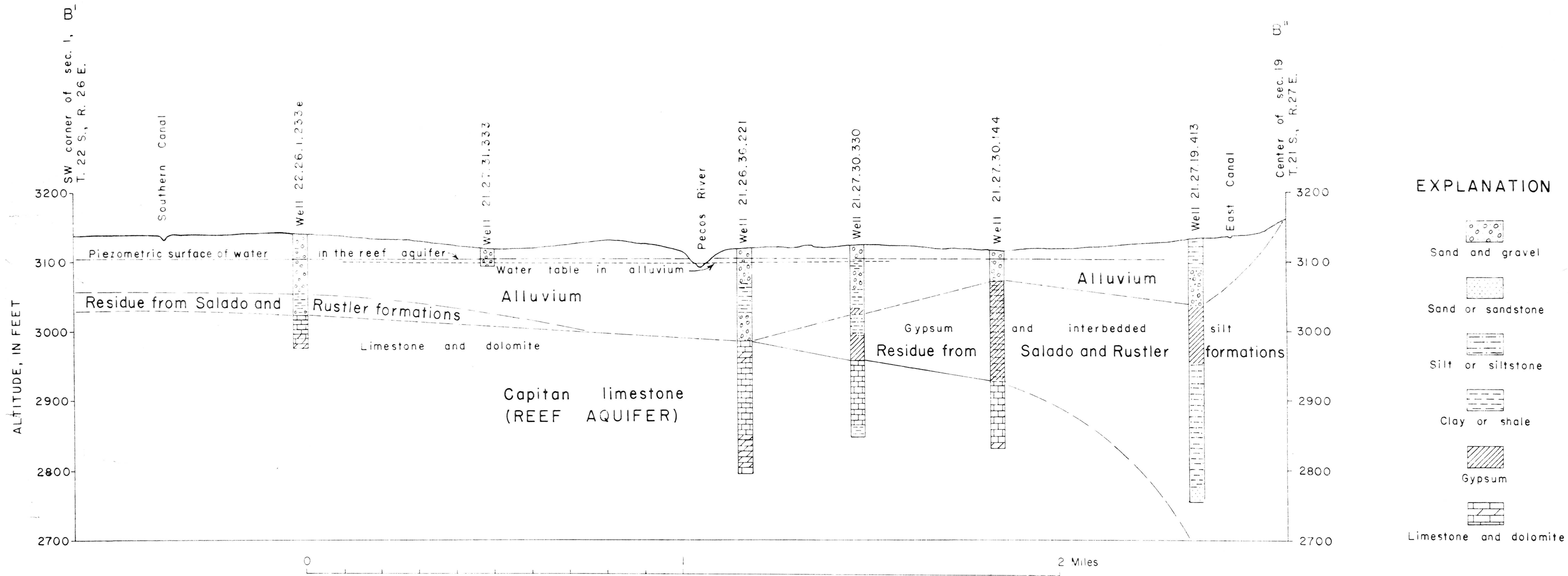
Figure 20.--Diagram showing geologic and hydrologic cross section B'-B'' from the vicinity of the Carlsbad city well field through La Huerta, Eddy County, N. Mex.
