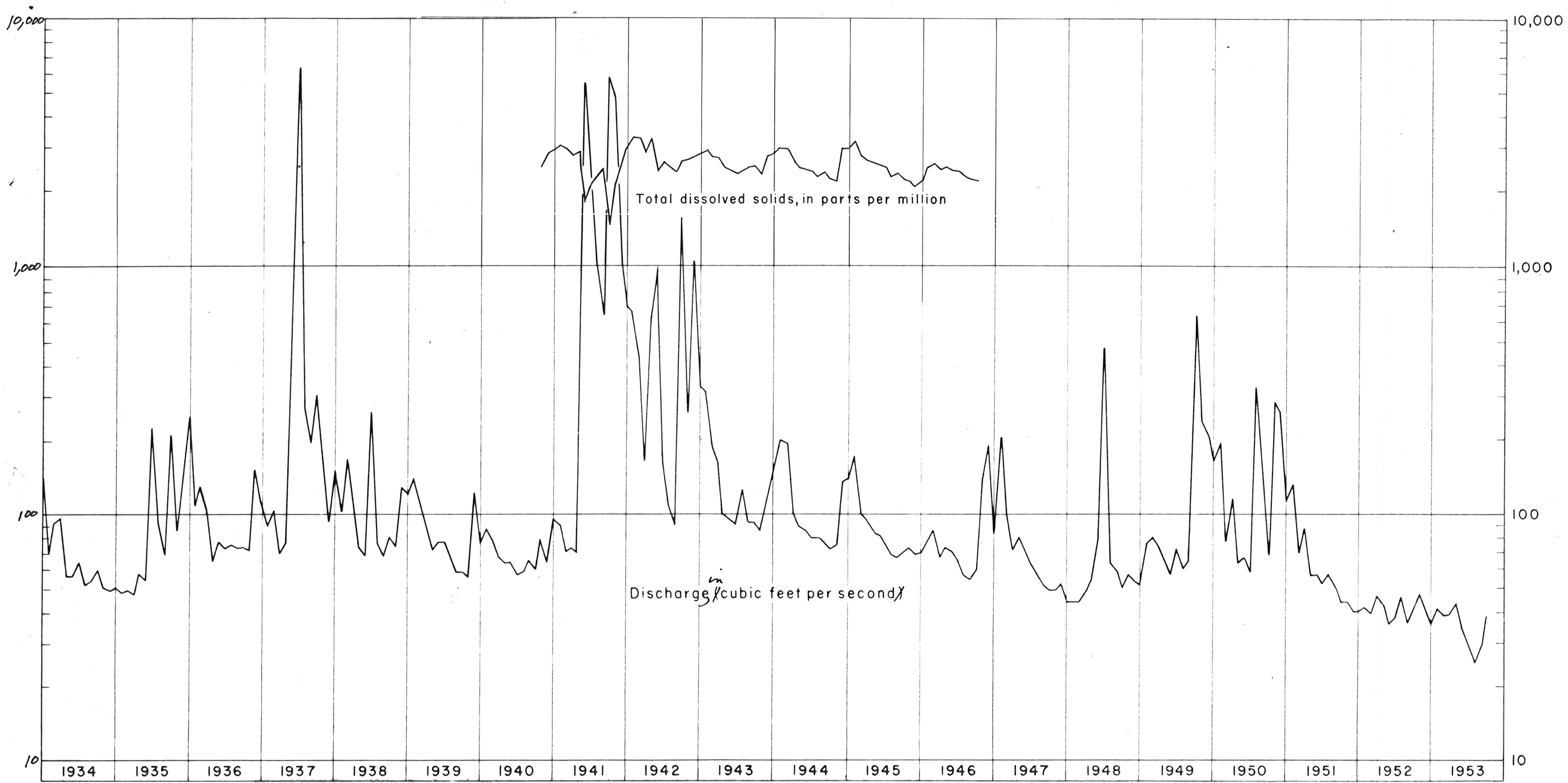
Figure 46.—Graphs showing monthly mean discharge of and total dissolved solids in the Pecos River at Carlsbad, Eddy County, N. Mex.
