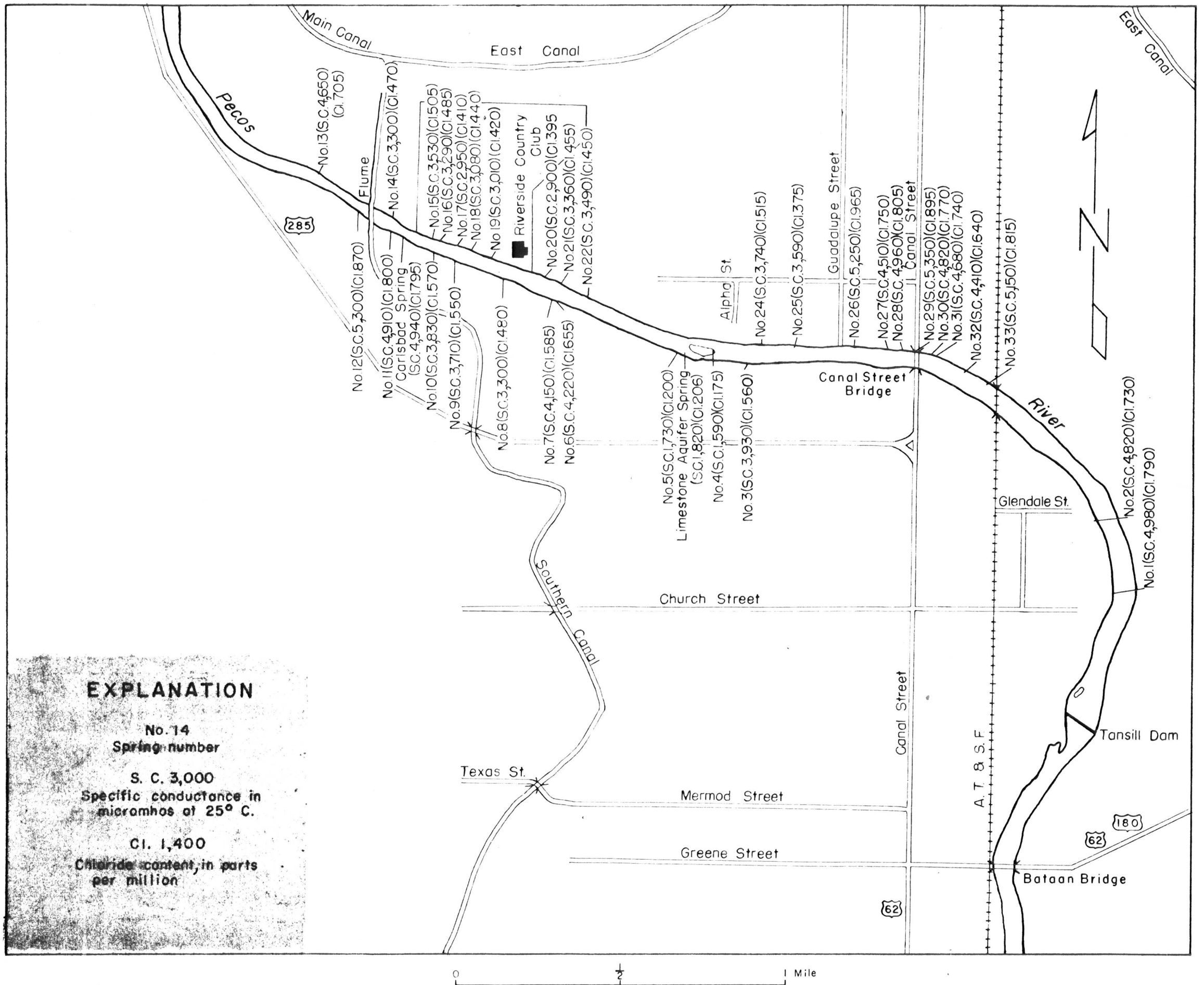
Figure 24. -- Map showing location of springs and analyses of water, Carlsbad Springs area, Eddy County, N. Mex.
