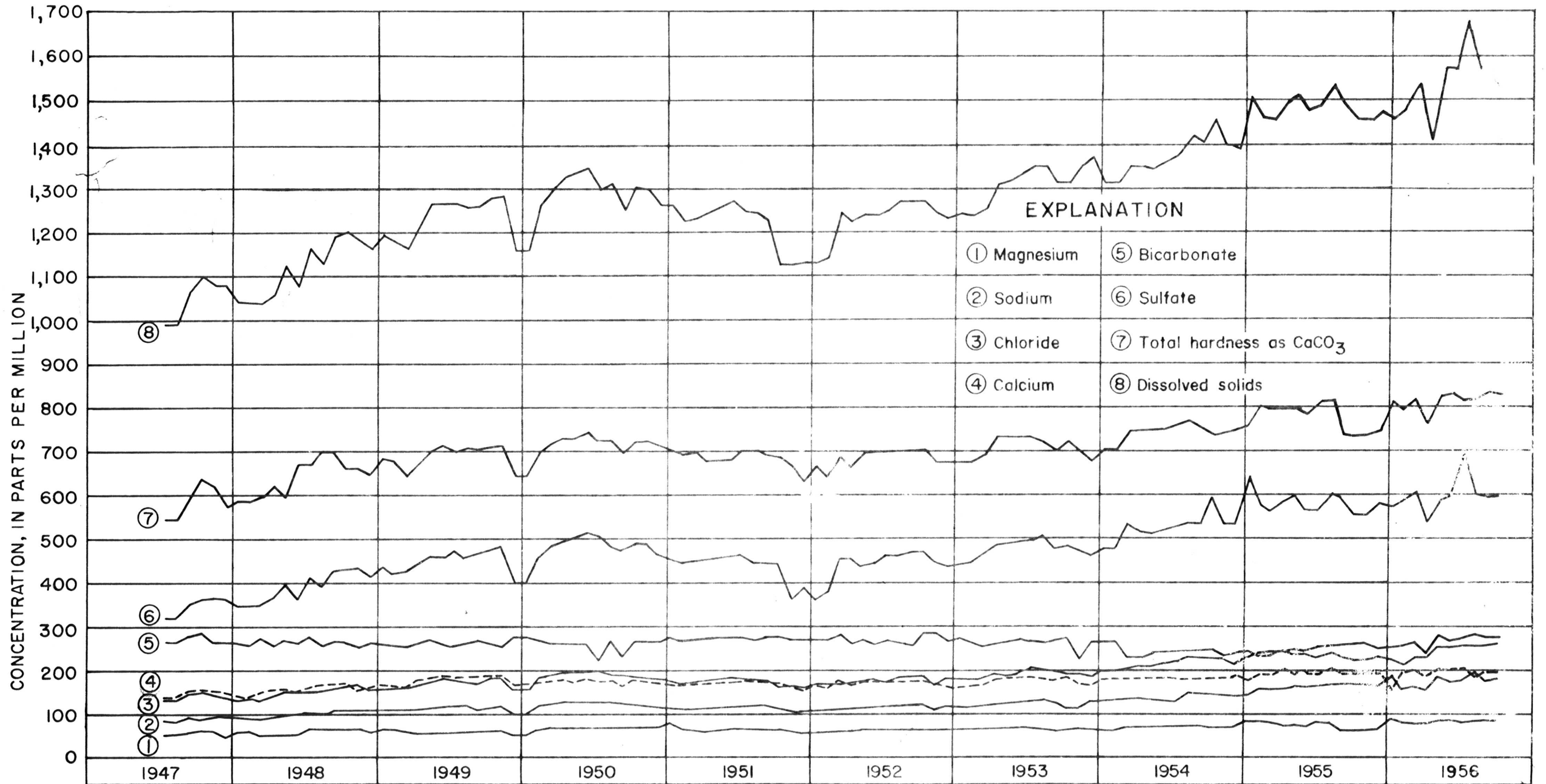
Figure 50.--Graph showing monthly chemical analyses of water pumped from the reef aquifer for industrial use during period 1947-56 from wells 21.27.30.434 and 21.27.30.434a. (Analyses by International Mineral and Chemical Corp., Carlsbad, N. Mex.; owner.)
