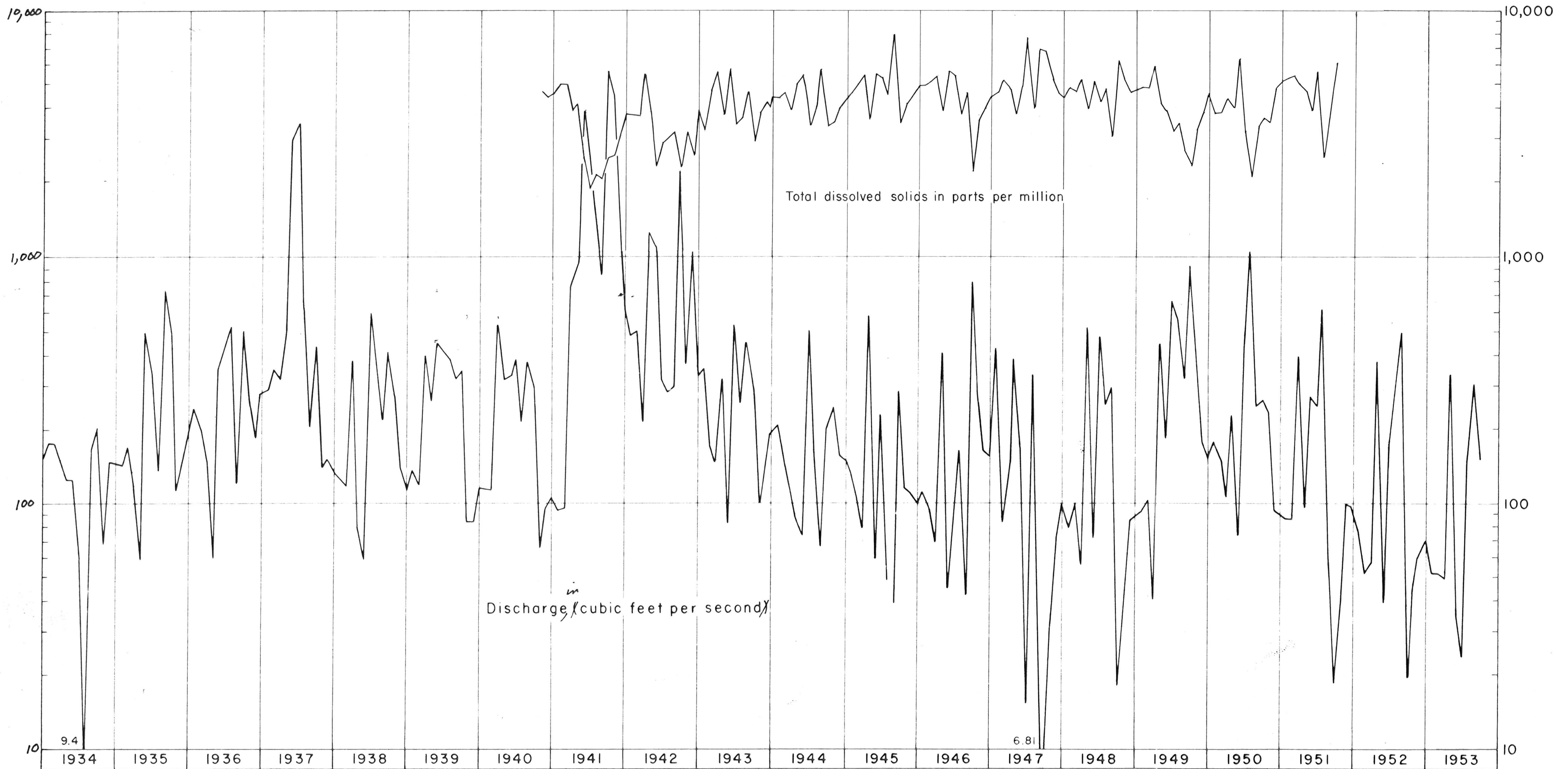
Figure 45.--Graphs showing monthly mean discharge of and total dissolved solids in the Pecos River at Artesia, Eddy County, N. Mex.
