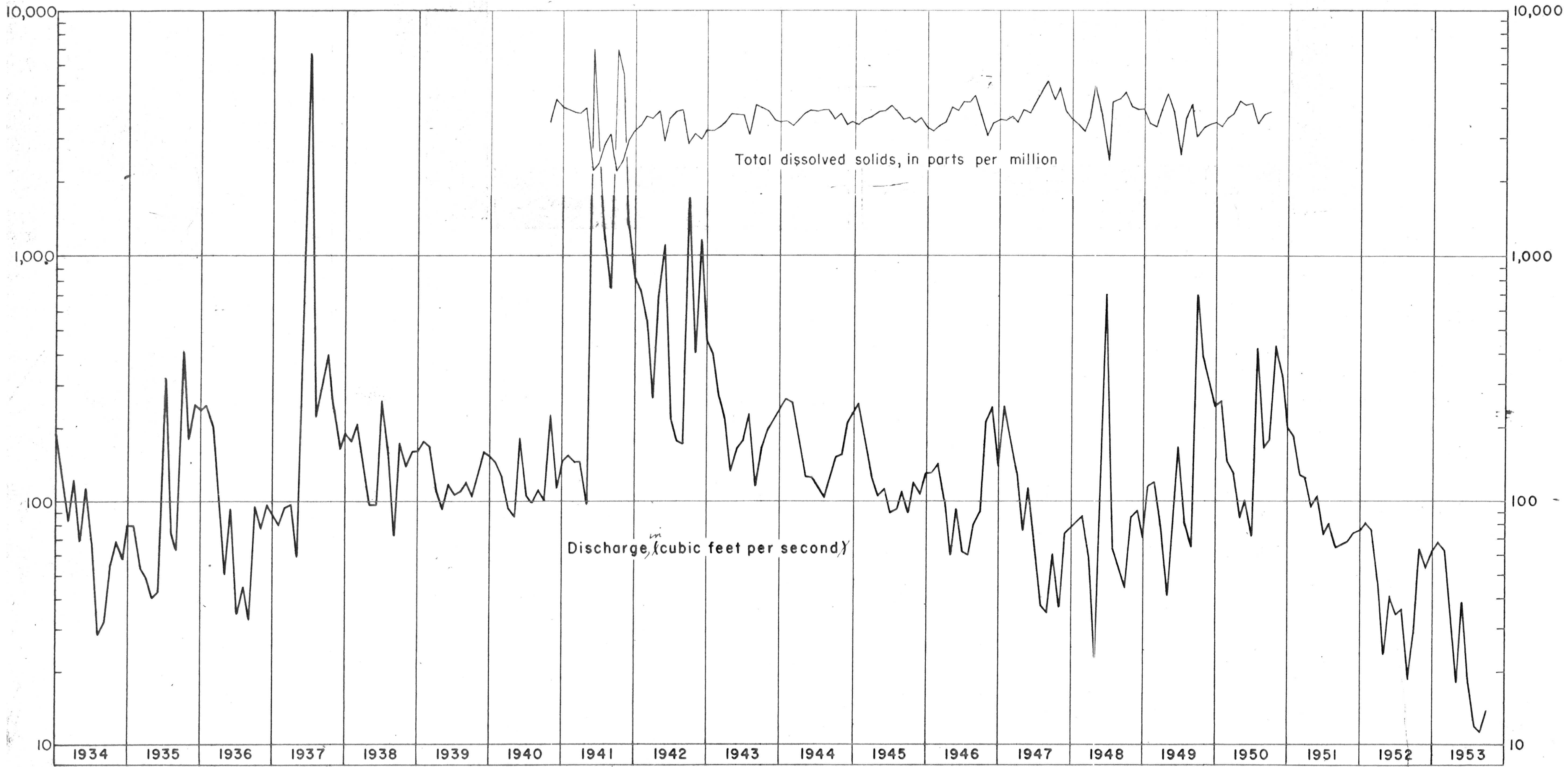
Figure 47.—Graphs showing monthly mean discharge of and total dissolved solids in the Pecos River at Malaga, Eddy County, N. Mex.
