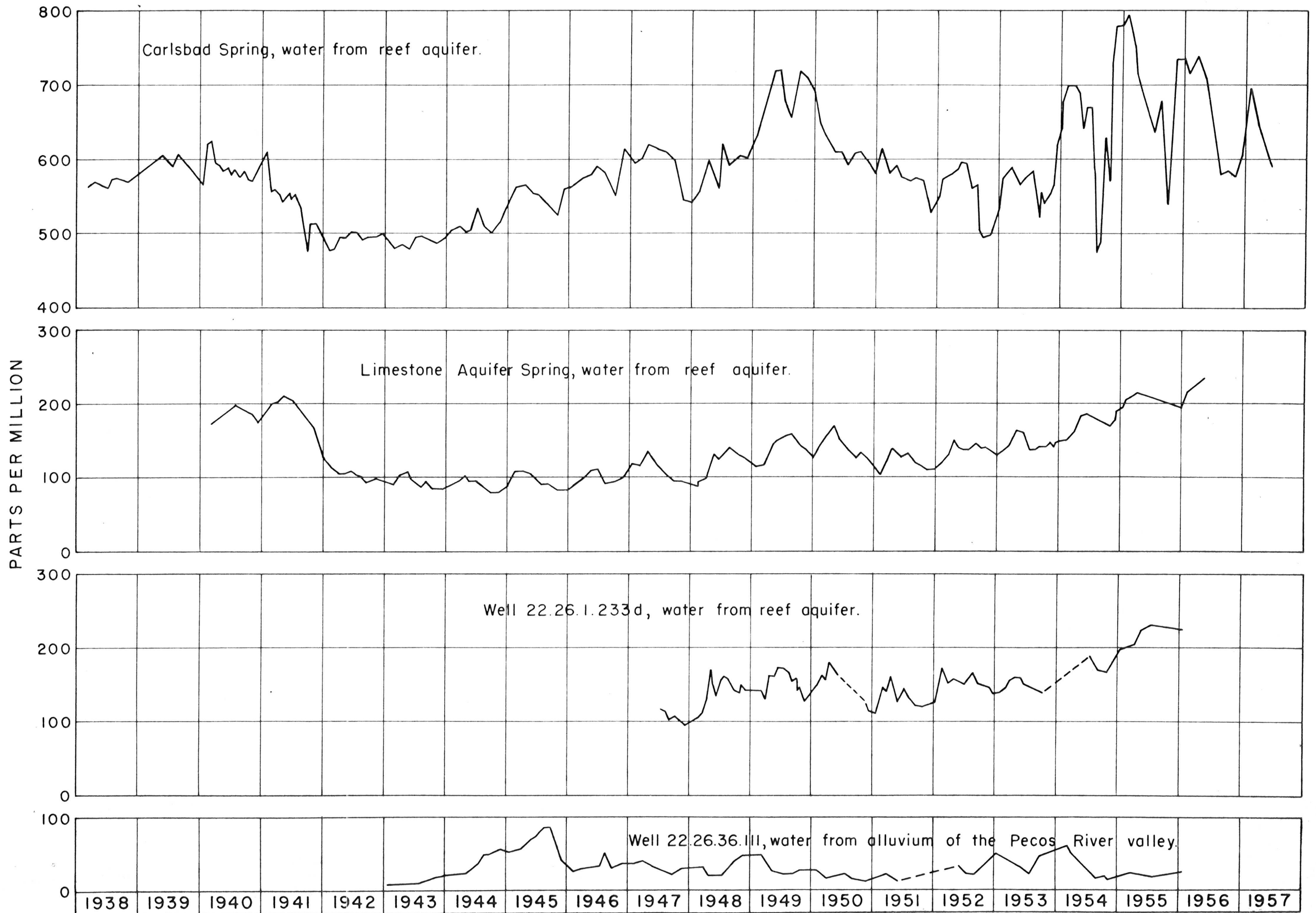
Figure 51.--Graphs showing chloride content in water from selected springs and wells in the vicinity of Carlsbad, Eddy County, N. Mex., 1938-57.
