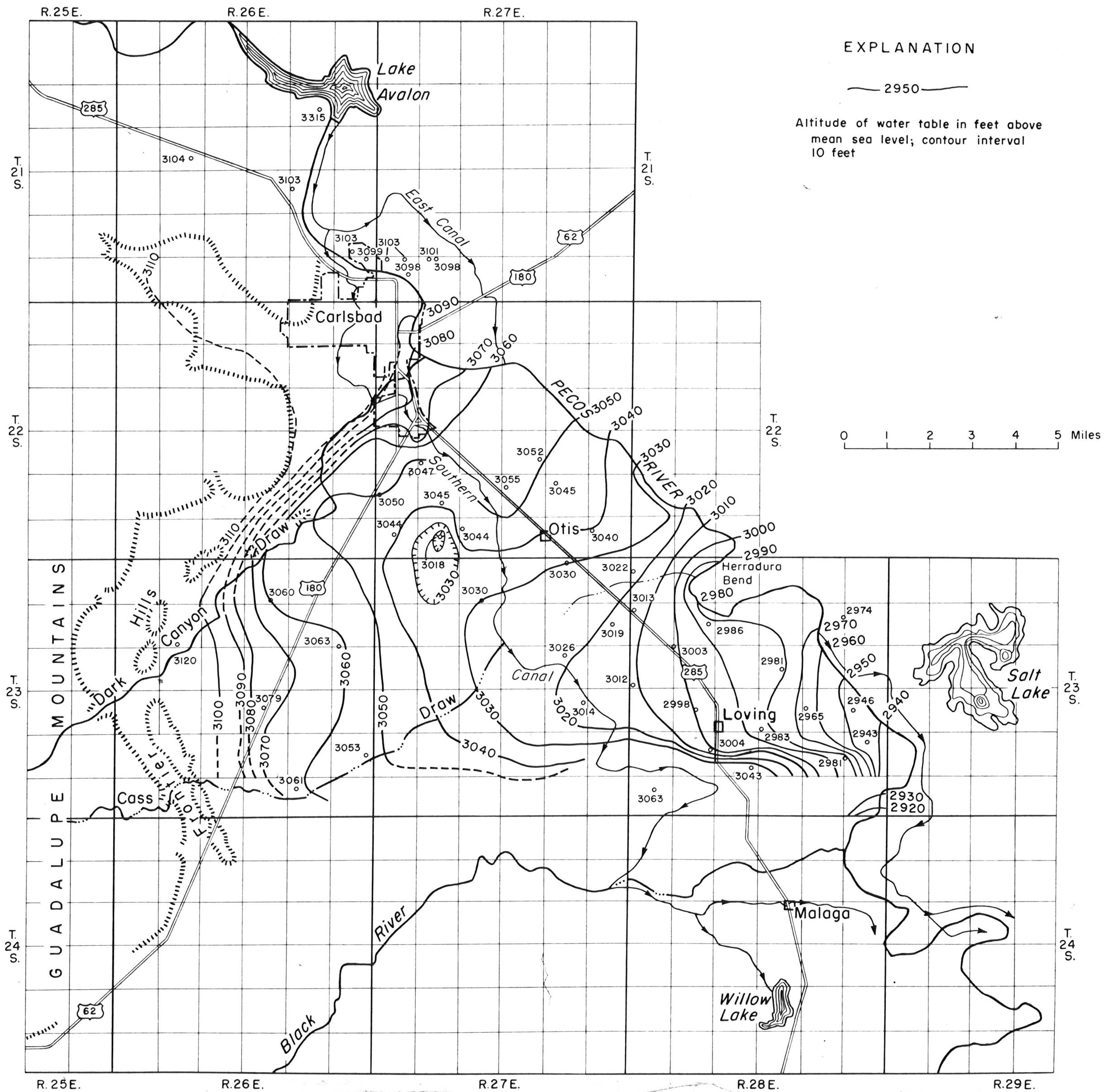
Figure 34.--Map showing configuration of the main water table in the alluvium of the Pecos River valley south of Carlsbad, Eddy County, N. Mex., during January 1954.
