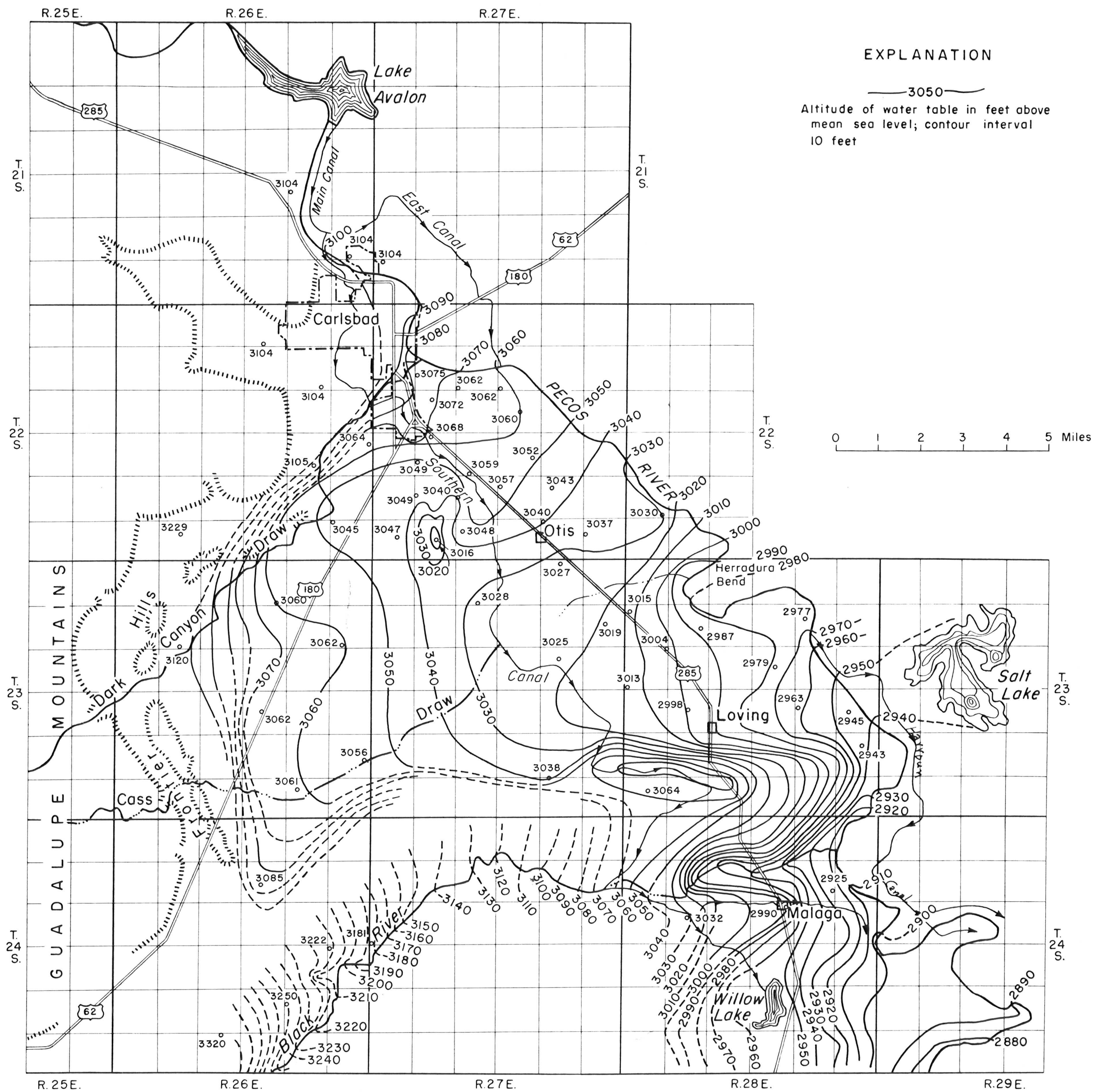
Figure 35.--Map showing configuration of the main water table in the alluvium of the Pecos River valley south of Carlsbad, Eddy County, N. Mex., during January 1955.
