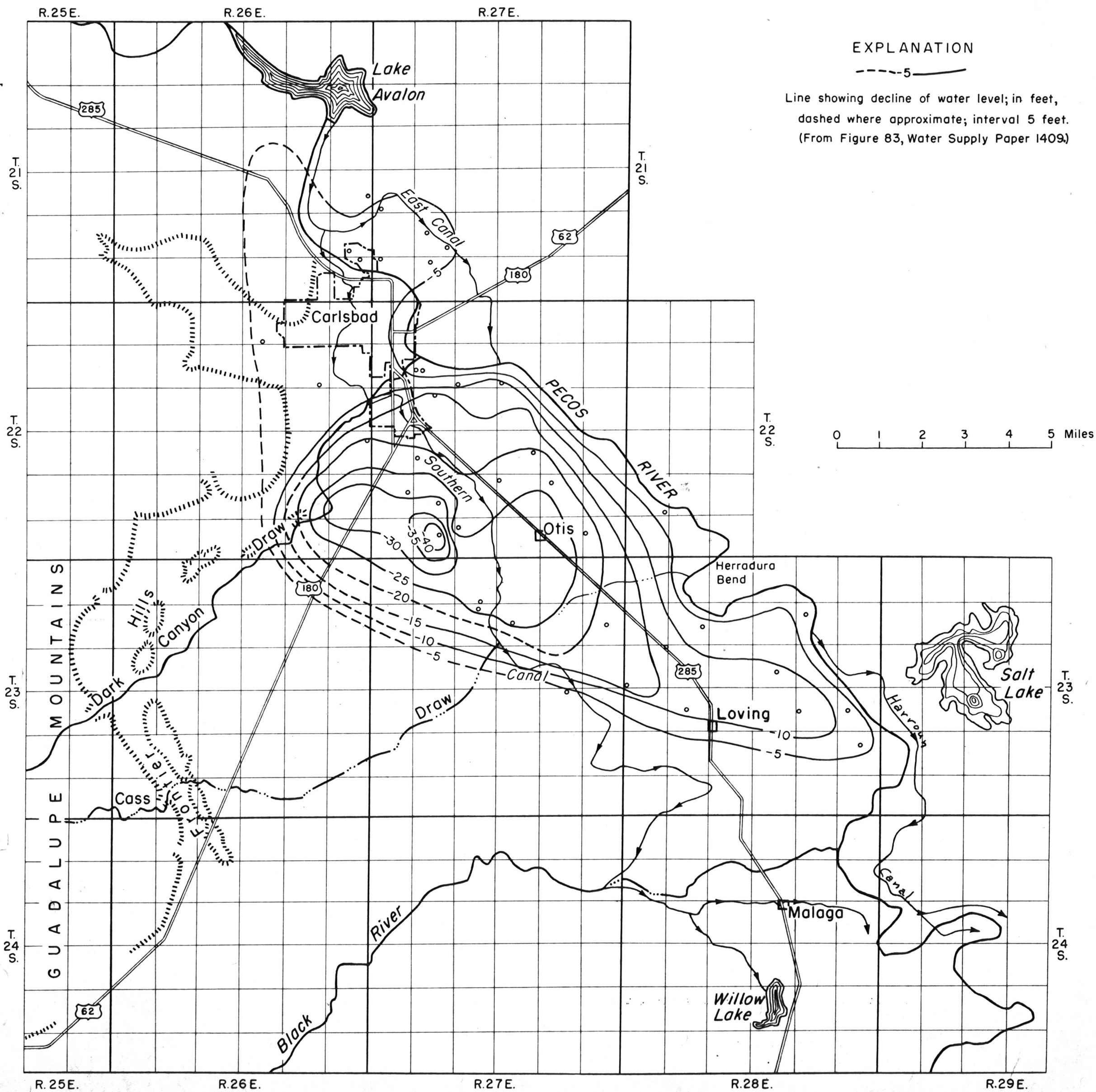
Figure 40.--Map showing change in ground-water level in the Carlsbad area, Eddy County, N. Mex., from January 1950 to January 1955.
