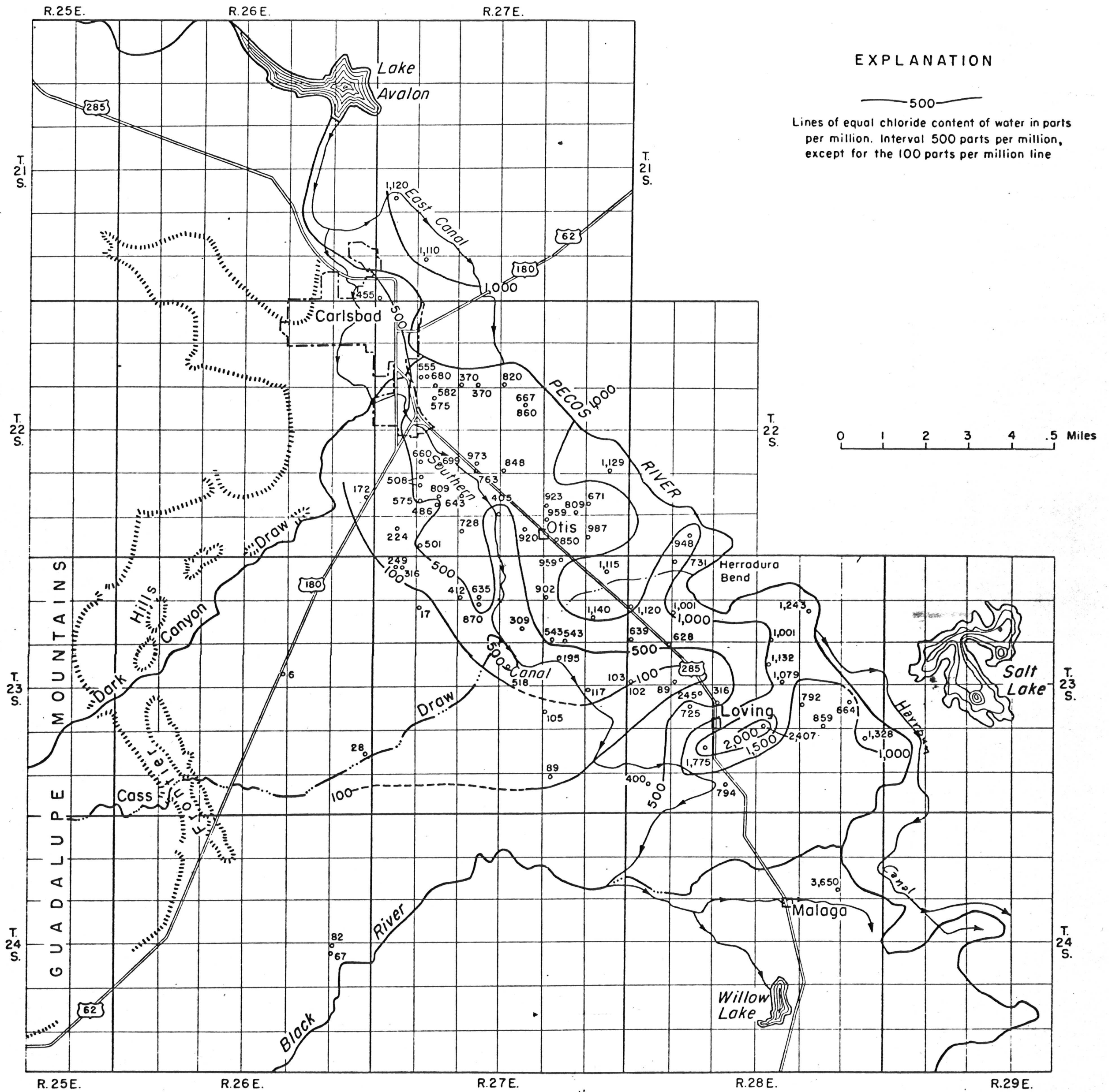
Figure 53.--Map showing chloride content of ground water in the of the Pecos River valley alluvium south of Carlsbad, Eddy County, N. Mex. Lines representing equal chloride content are generalized. Data shown are analyses of samples collected from 1953-55.
