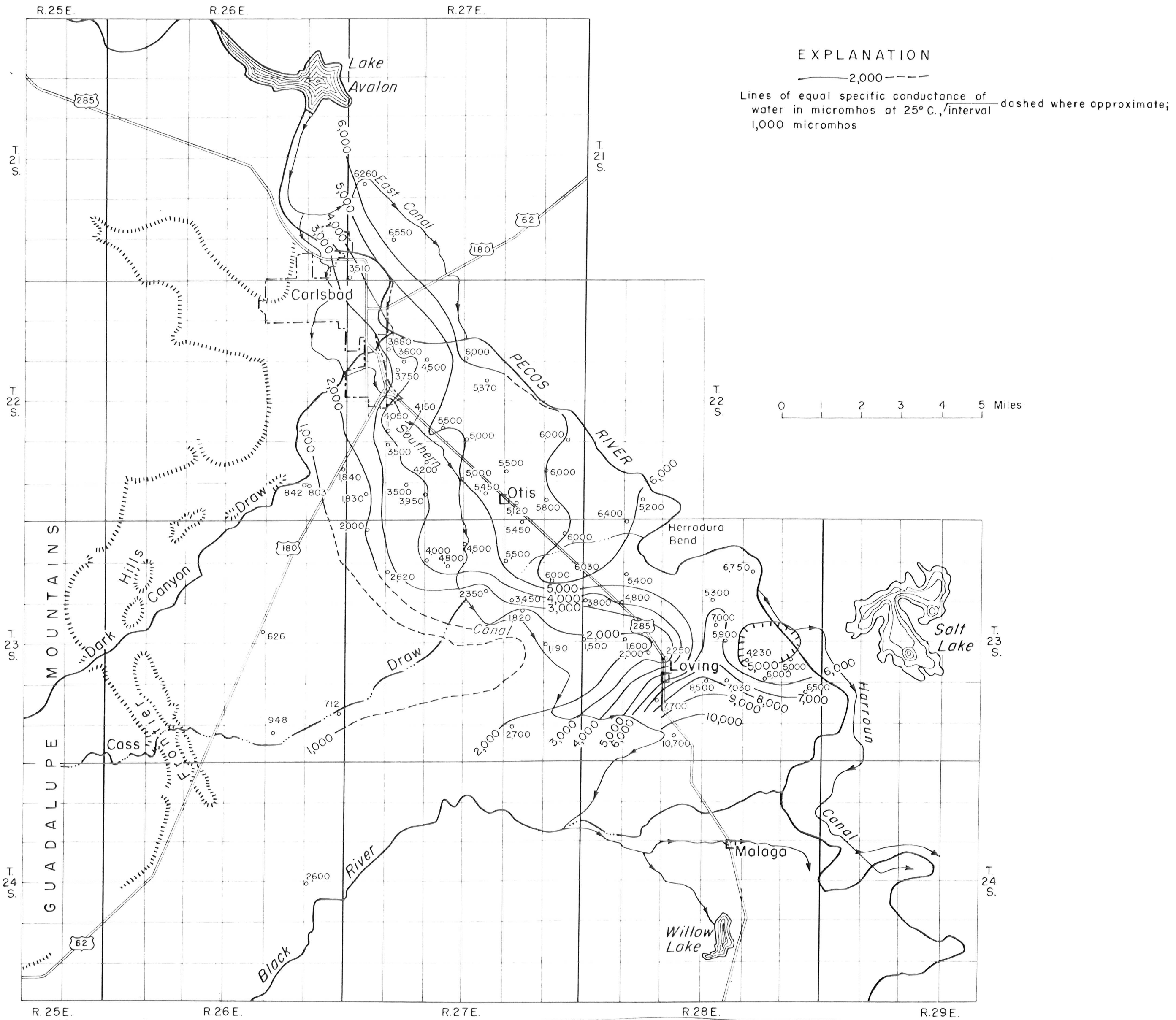
Figure 52.—Map showing specific conductance of ground water in the alluvium of the Pecos River valley south of Carlsbad, Eddy County, N. Mex. Lines representing equal specific conductance are generalized. Data shown are analyses of samples collected from 1953-55.
