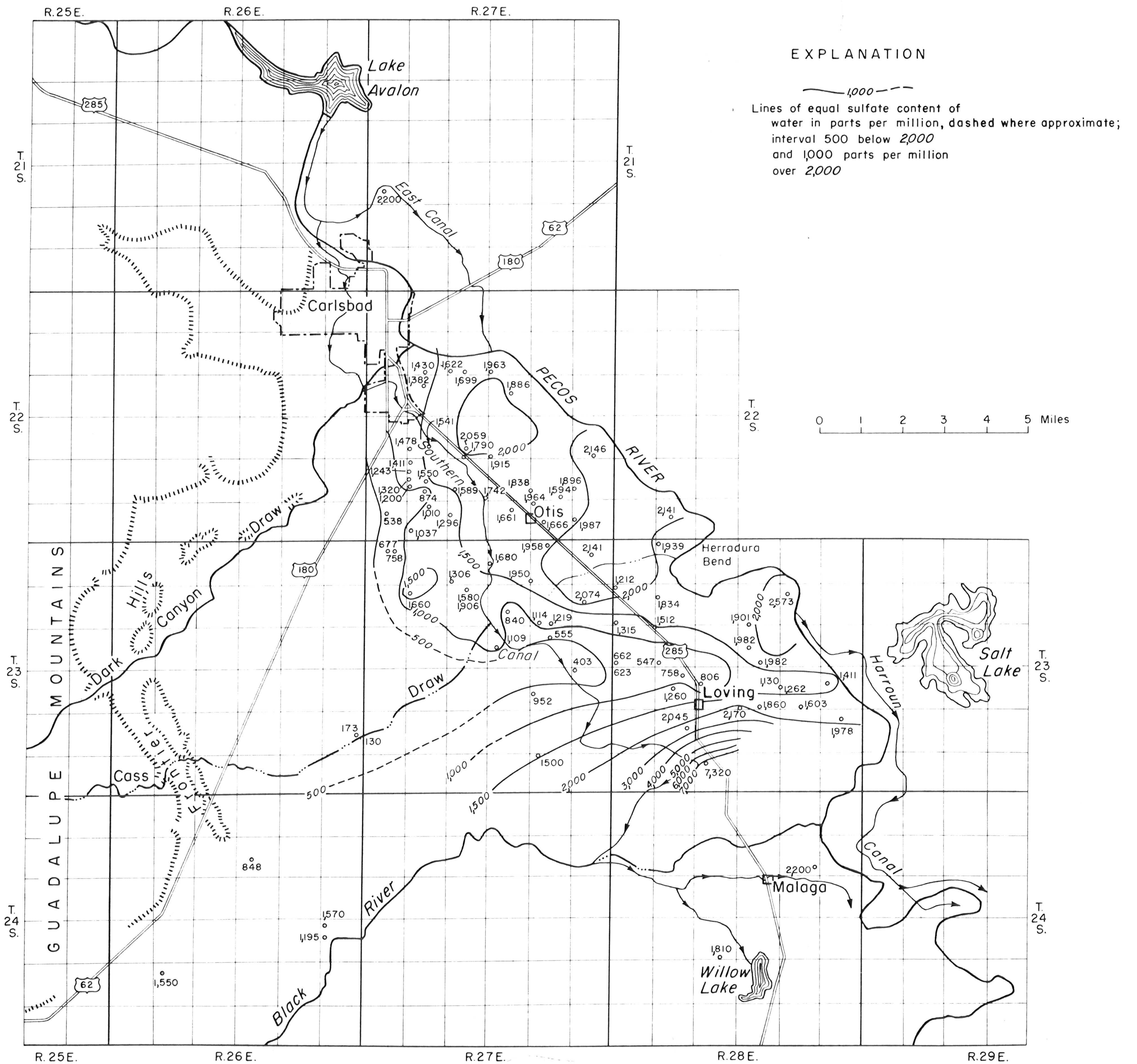
Figure 54.--Map showing sulfate content of ground water in the alluvium of the Pecos River valley south of Carlsbad, Eddy County, N. Mex. Lines representing equal sulfate content are generalized. Data shown are analyses of samples collected from 1953-55
