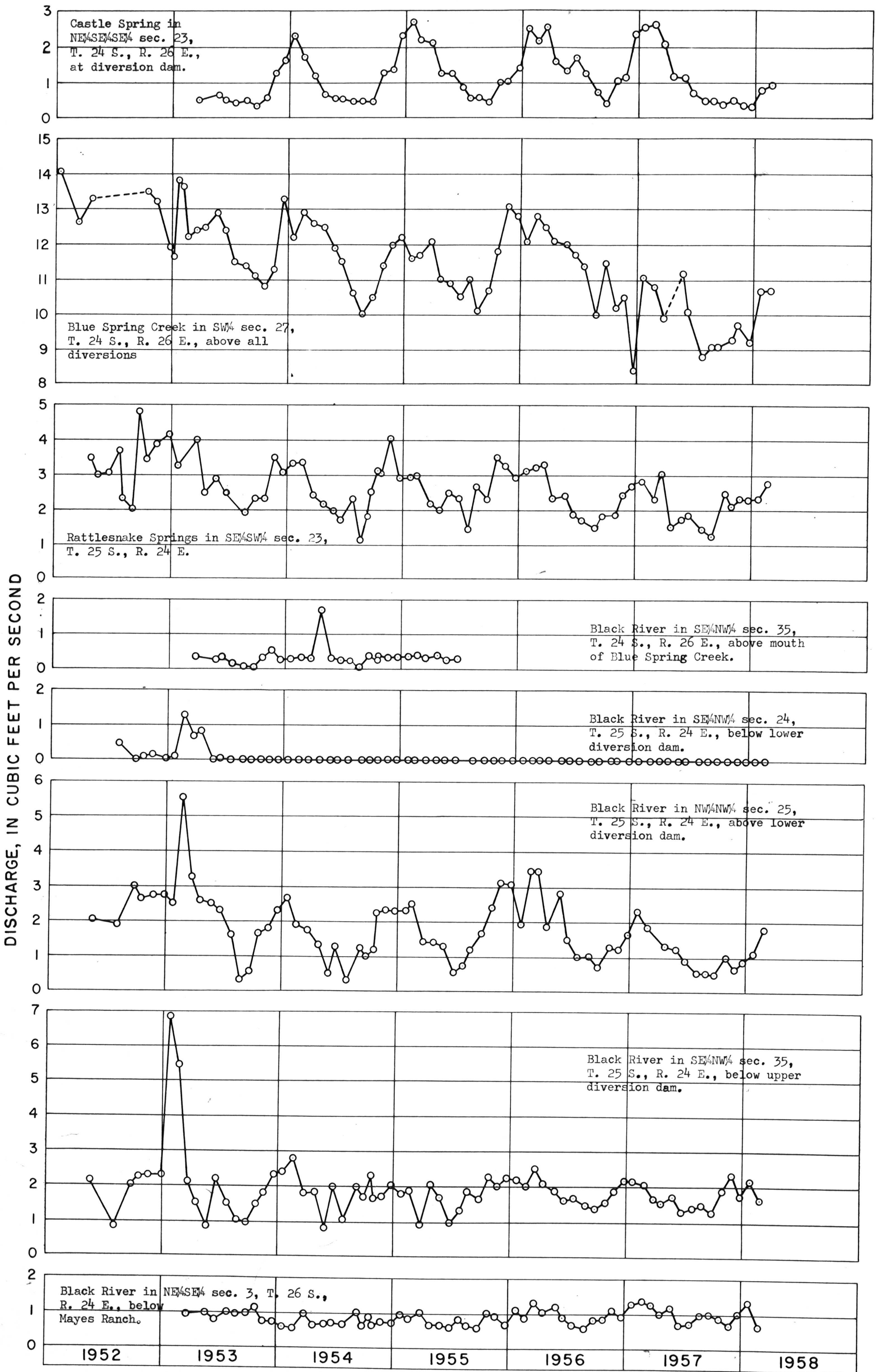
Figure 44.—Hydrographs of spring and stream discharge in the upper Black River valley, Eddy County, N. Mex., 1952-58. Data obtained from U.S.G.S. Water-Supply Papers and field records.
