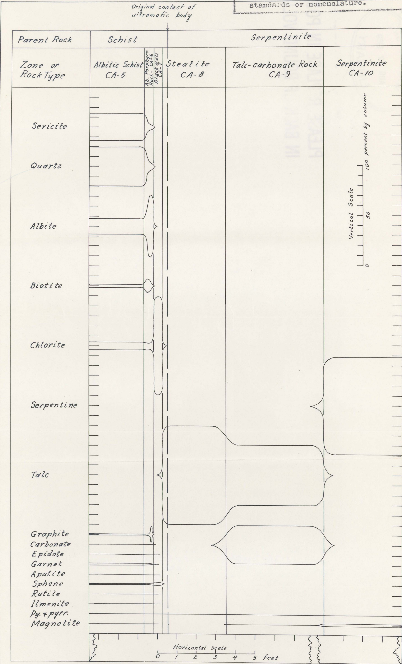
Figure 4.-- Variation diagram, based upon modes (volume percent) of an idealized suite across the contact of an ultramafic body (table 2-B), showing the mineralogical changes that occurred in the rocks during steatitization.
