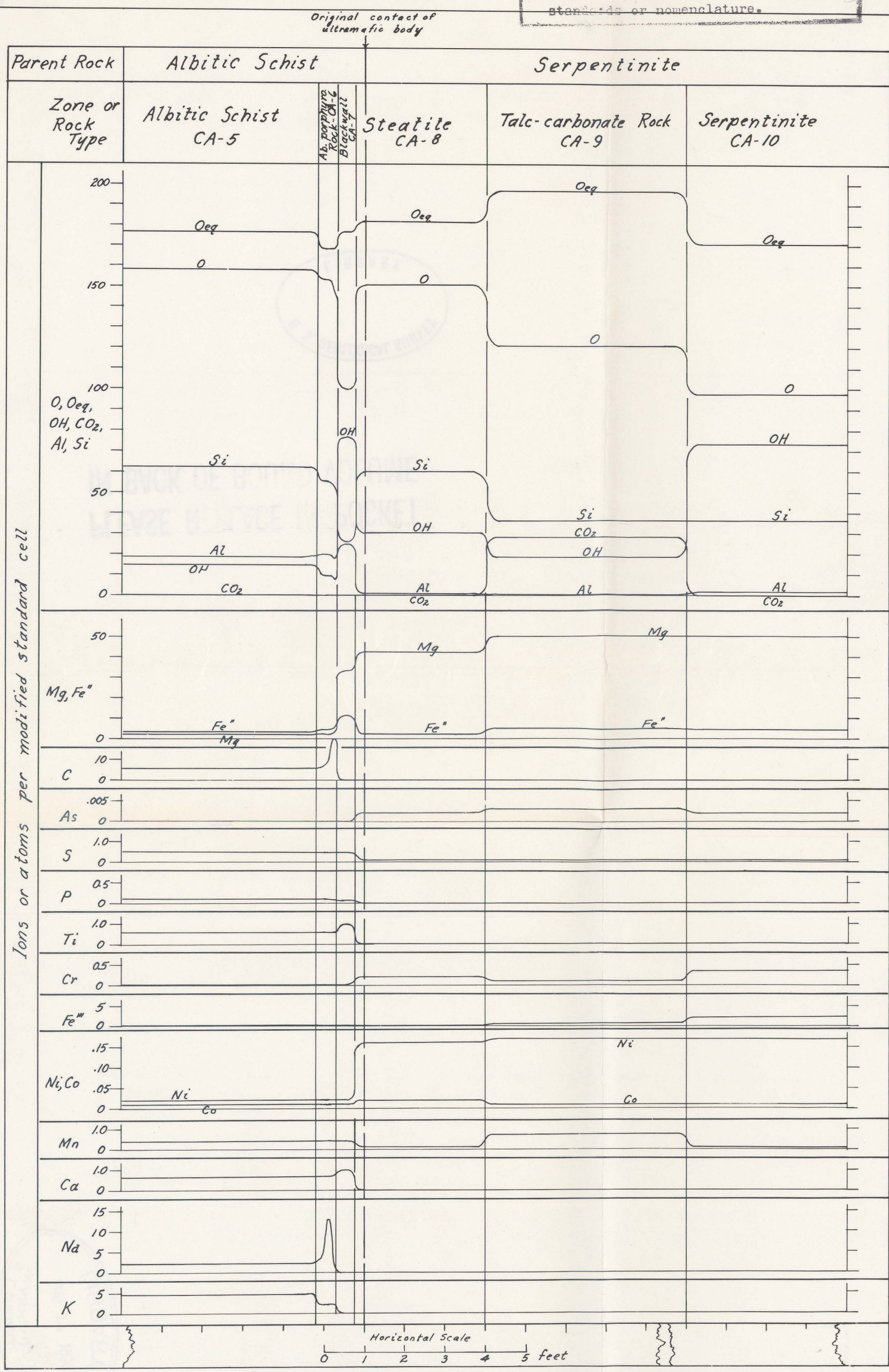
Figure 5.— Variation diagram, based upon rock formulas determined from the modified standard cell (table 2-C), of an idealized suite of rocks across the contact of an ultramafic body, showing the chemical changes that occurred in the rocks during steatitization.
