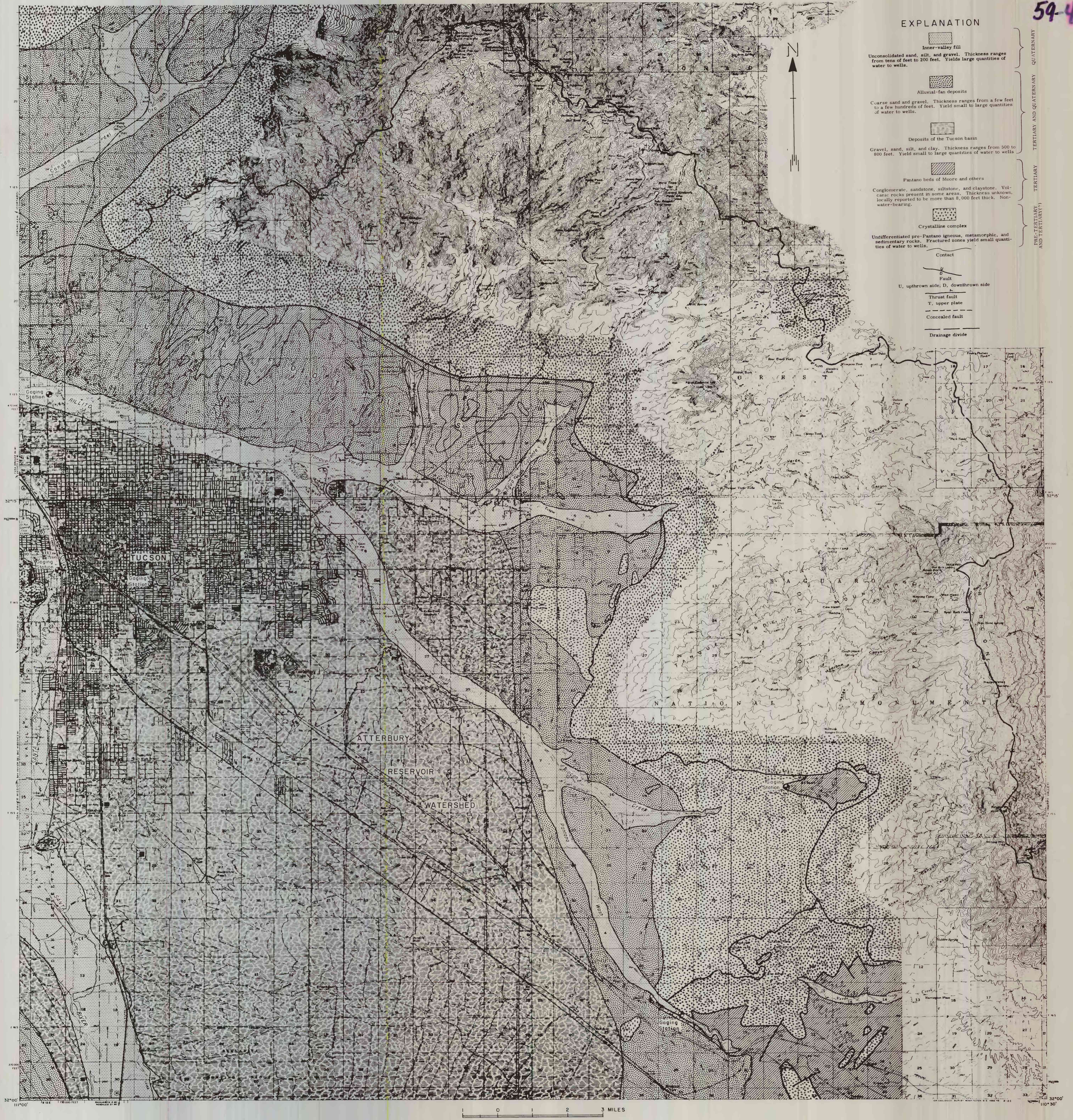
FIGURE 3.-- GEOLOGIC MAP OF THE TUCSON BASIN AREA.
