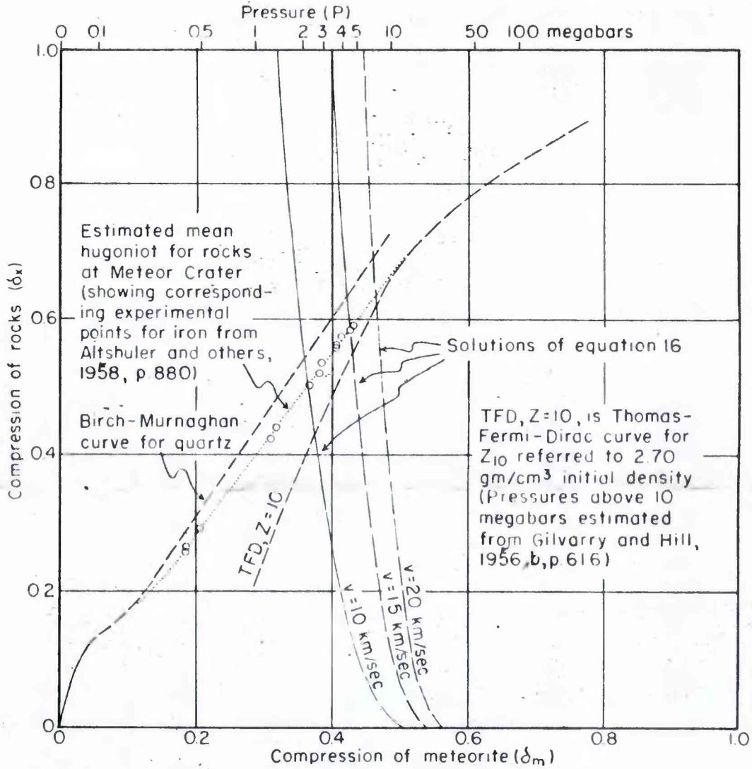
✓ FIGURE 5.—COMPRESSION OF ROCKS AT METEOR CRATER, ARIZONA, AS A FUNCTION OF COMPRESSION OF THE METEORITE AND OF PRESSURE.
