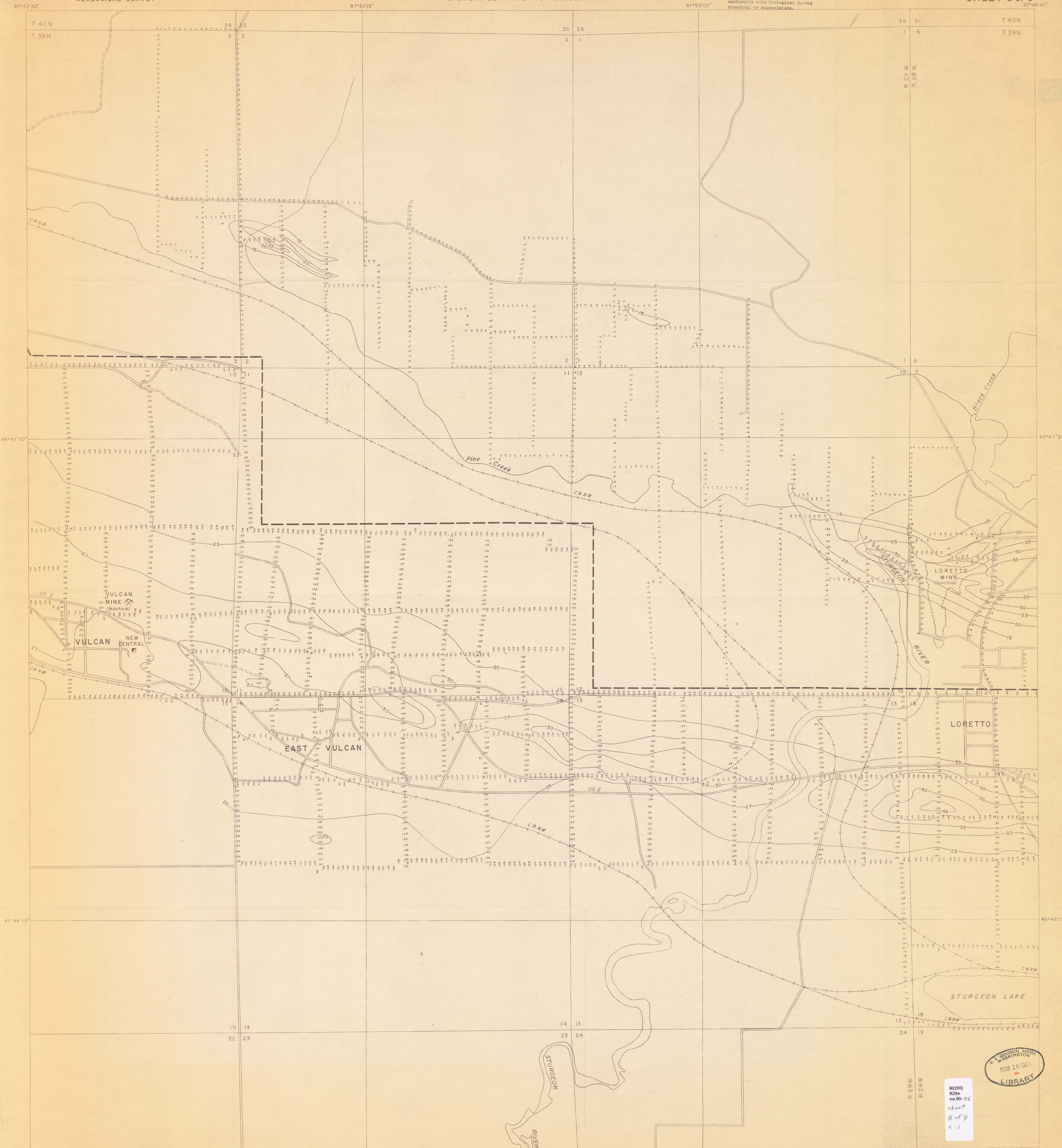
MAP SHOWING MAGNETIC DATA OF SOUTHERN DICKINSON COUNTY, MICHIGAN
