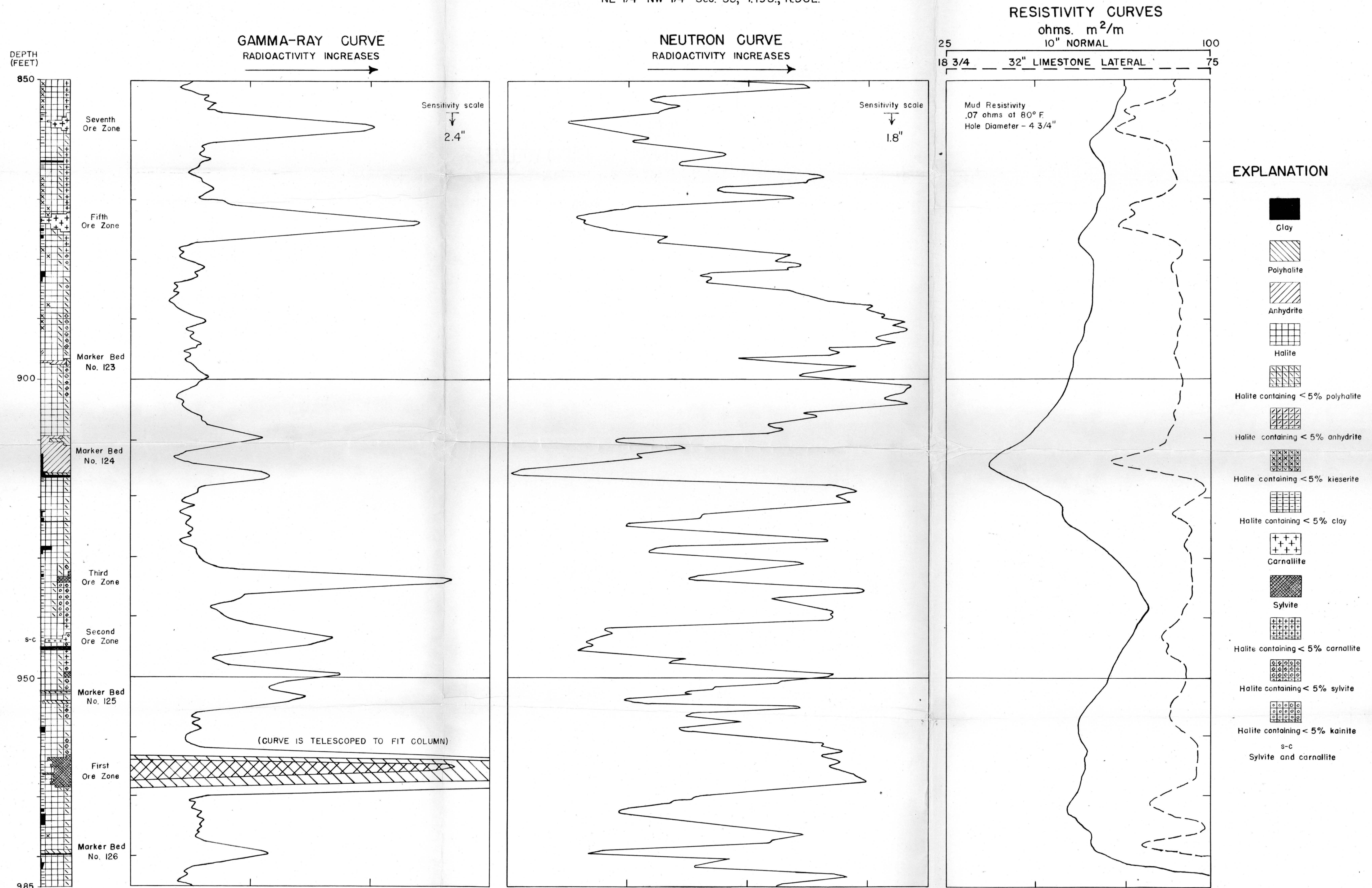
Figure 3. Lithologic, gamma-ray, neutron, and electrical resistivity logs, showing correlation of geology and anomalies obtained with well logging instruments.
