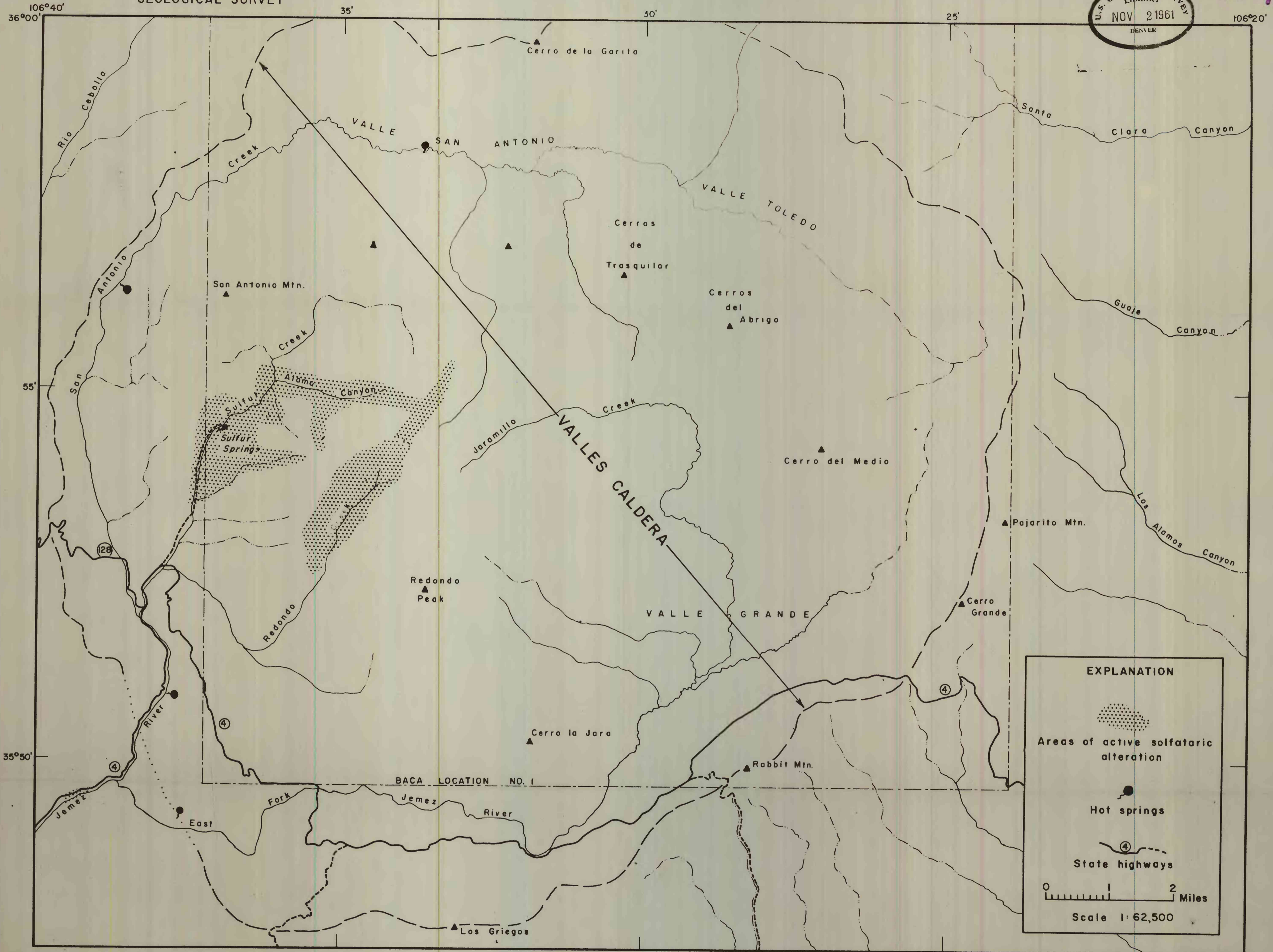
HOT SPRINGS AND SOLFATARIC AREAS IN THE VALLES CALDERA, JEMEZ MOUNTAINS, N. MEX.
