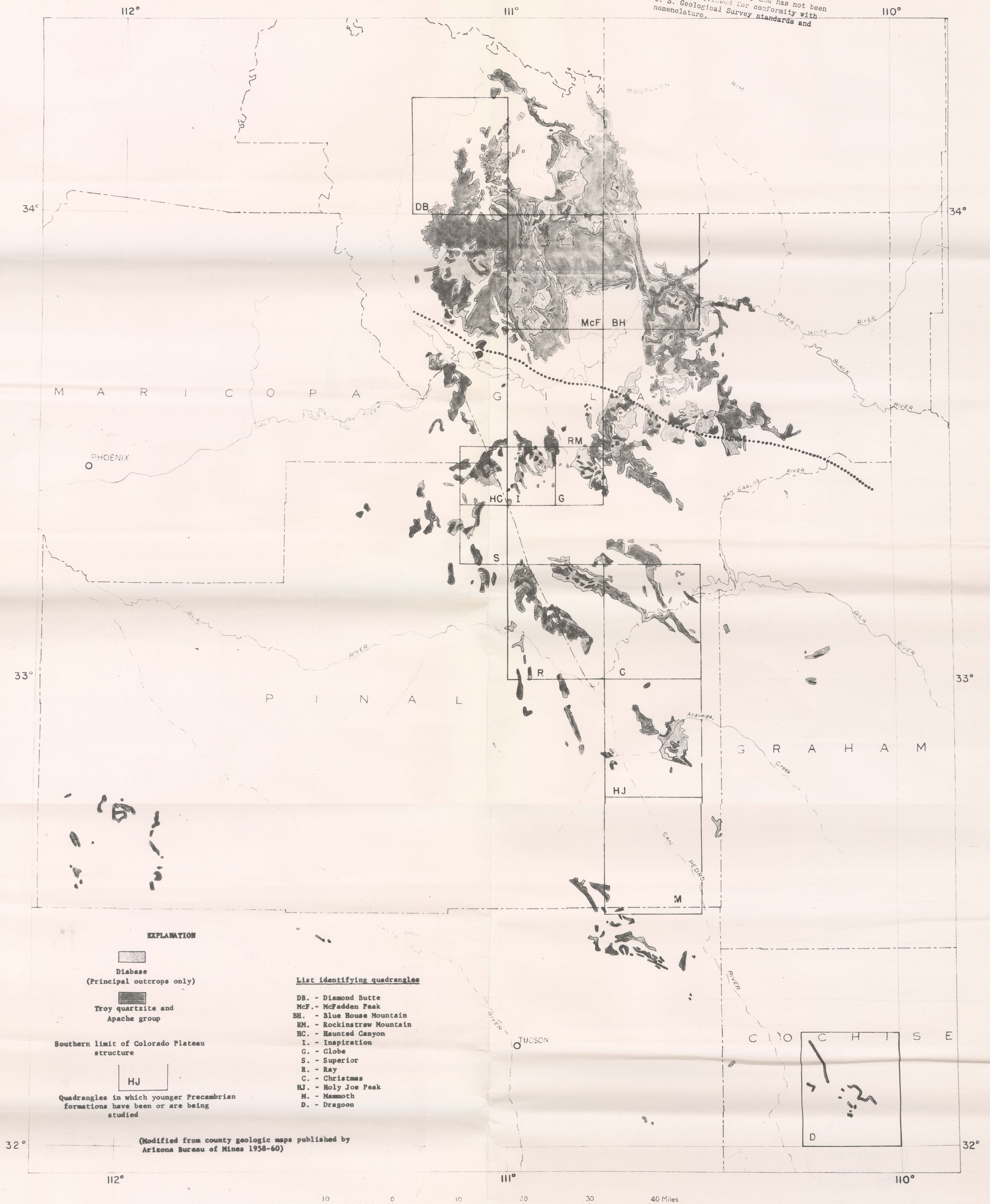
FIGURE 2. MAP SHOWING OUTCROPS OF YOUNGER PRECAMBRIAN STRATA AND COEXTENSIVE DIABASE INTRUSIONS IN SOUTHEASTERN ARIZONA
